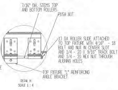
DETAIL H SCALE 1:4
