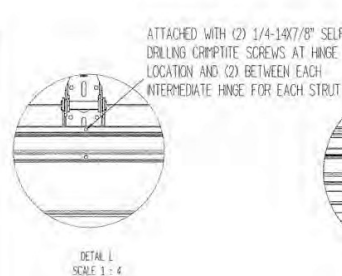
DETAIL L SCALE 1:4
