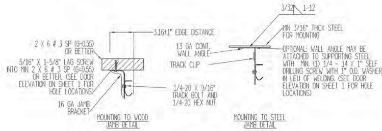
WOOD MOUNTED TO #3 SOUTHERN PINE SUBSTRATE
