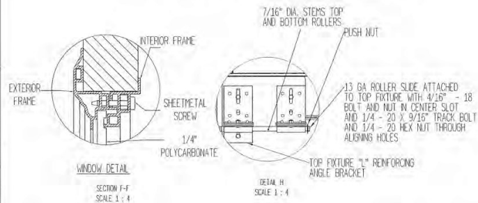
DETAIL H SCALE 1:4
