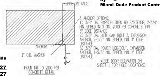
WOOD MOUNTED TO 2000 PSI CONCRETE DETAIL
