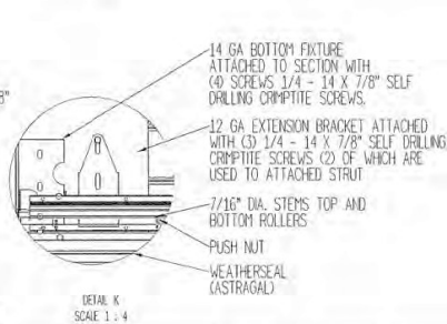
DETAIL K SCALE 1:4
