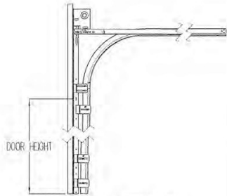
STANDARD LIFT TRACK DETAIL
