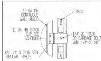
TYPICAL TRACK CLIP BOLTING DETAIL
