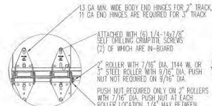
DETAIL Q SCALE 1:4
