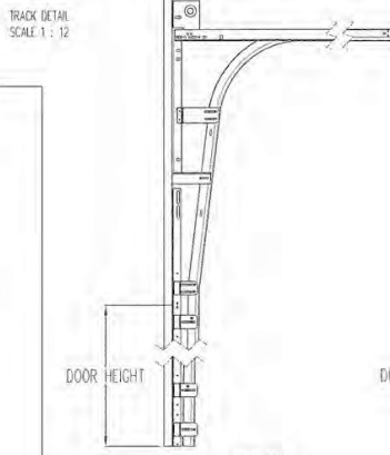
HIGH LIFT TRACK DETAIL
