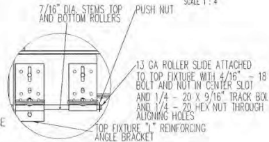
DETAIL O SCALE 1:4
