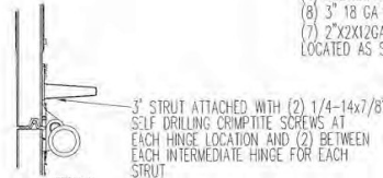
DETAIL N SCALE 1:4
