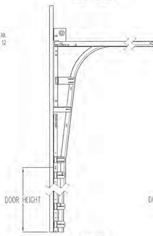
HIGH LIFT TRACK DETAIL
