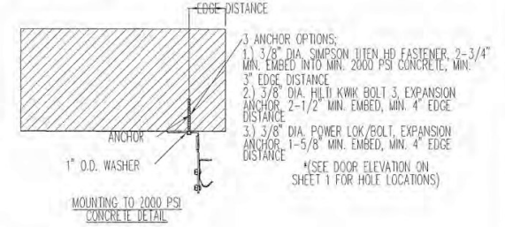
WOOD MOUNTED TO 2000 PSI CONCRETE DETAIL
