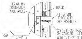
TYPICAL TRACK CLIP WELDING DETAIL
