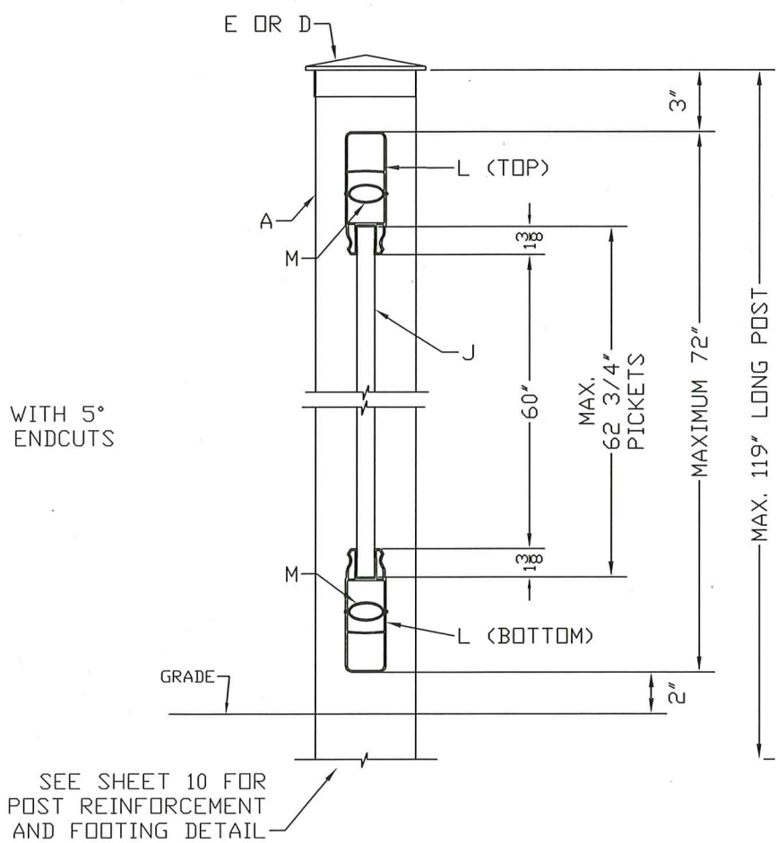
VERTICAL SECTION
