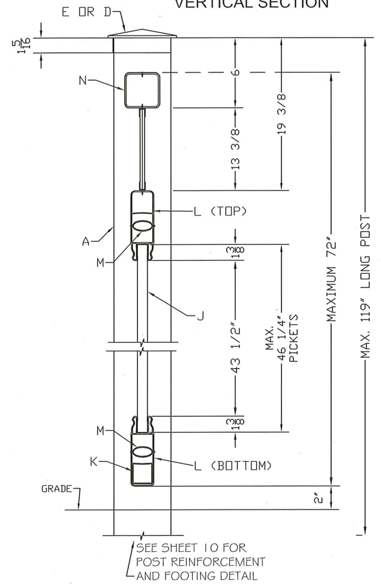
VERTICAL SECTION
