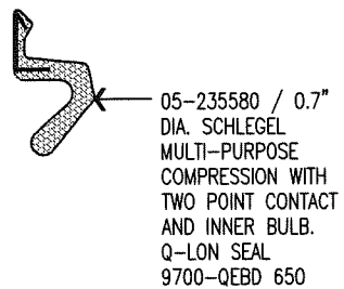
Y TYP. WEATHER STRIP FULL SCALE
