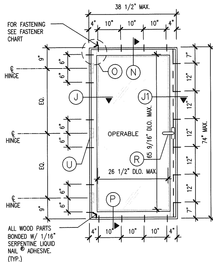
4A VENICE SERIES - OUTSWING SINGLE WOOD CASEMENT WINDOW SCALE: 1/2"=1'-0" X
