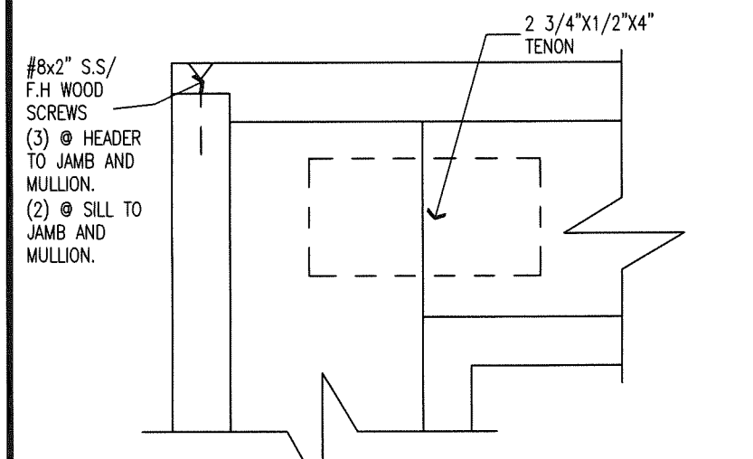
J WINDOW JAMB AT HINGE SIDE SCALE: 6"=1'-0"
