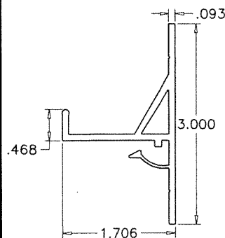
2 INTERMEDIATE ANCHOR
