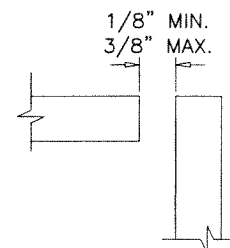
90° INSIDE CORNER
