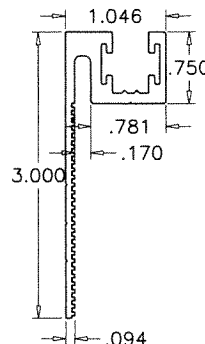
3 ULTRA ANCHOR
