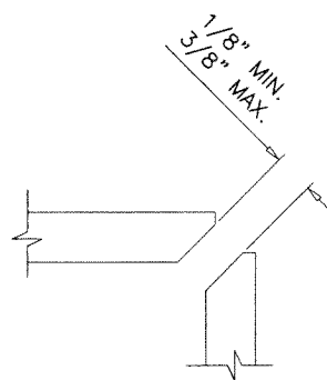
90° INSIDE CORNER
