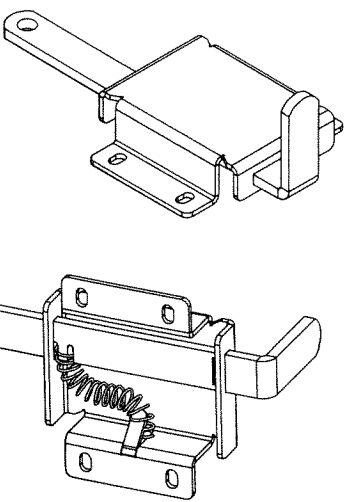
SLIDE LOCK ASSEMBLY
