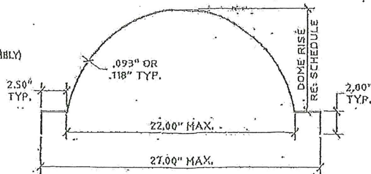
2 POLYCARBONATE DOME PROFILE (LOW PROFILE FLAT ROOF MOUNT) SCALE: 1-1/2" = 1' - 0"
