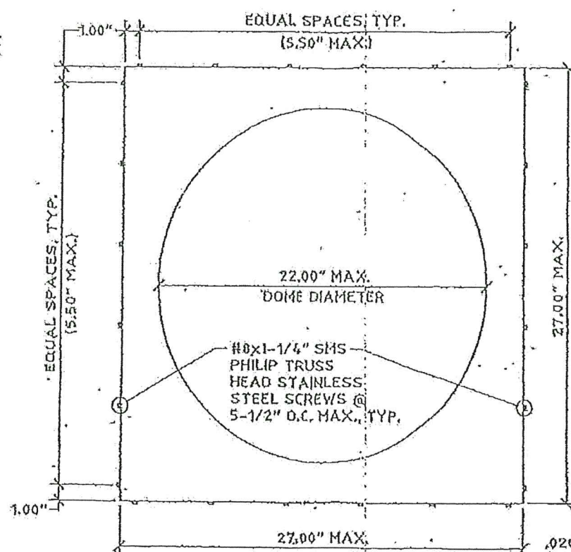
3 POLYCARBONATE DOME PLAN (LOW PROFILE FLAT ROOF MOUNT) SCALE: 1-1/2" = 1' - 0"
