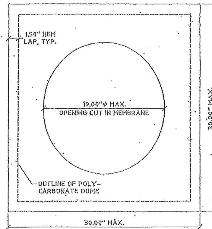
5 60 MIL. POLYVINYL CHLORIDE SINGLE-PLY MEMBRANE FLASHING BY SEAMAN CORP. APPROVED BY MDC N.O.A. # 00-1208.02 (LOW PROFILE FLAT ROOF MOUNT) SCALE: 1-1/2" = 1' - 0"
