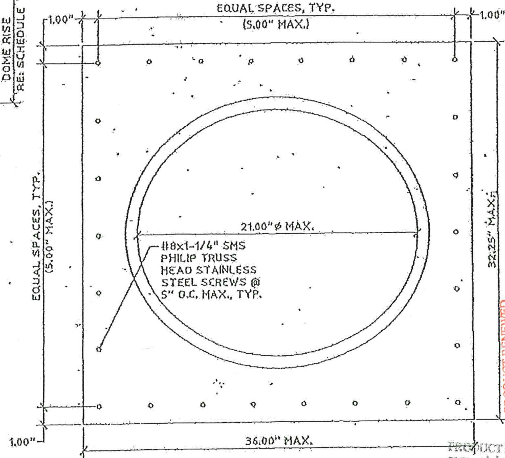
5 FLASHING PLAN (STANDARD ROOF MOUNT) SCALE: 1-1/2" = 1'-0"
