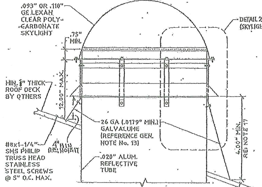
1 STANDARD FLAT ROOF MOUNT (STD MODEL) SCALE: 1-1/2" = 1'-0"
