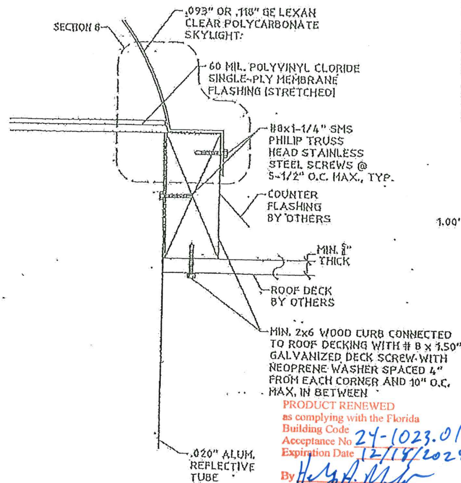
4 SKYLIGHT ASSEMBLY SCALE: 3\"/>
