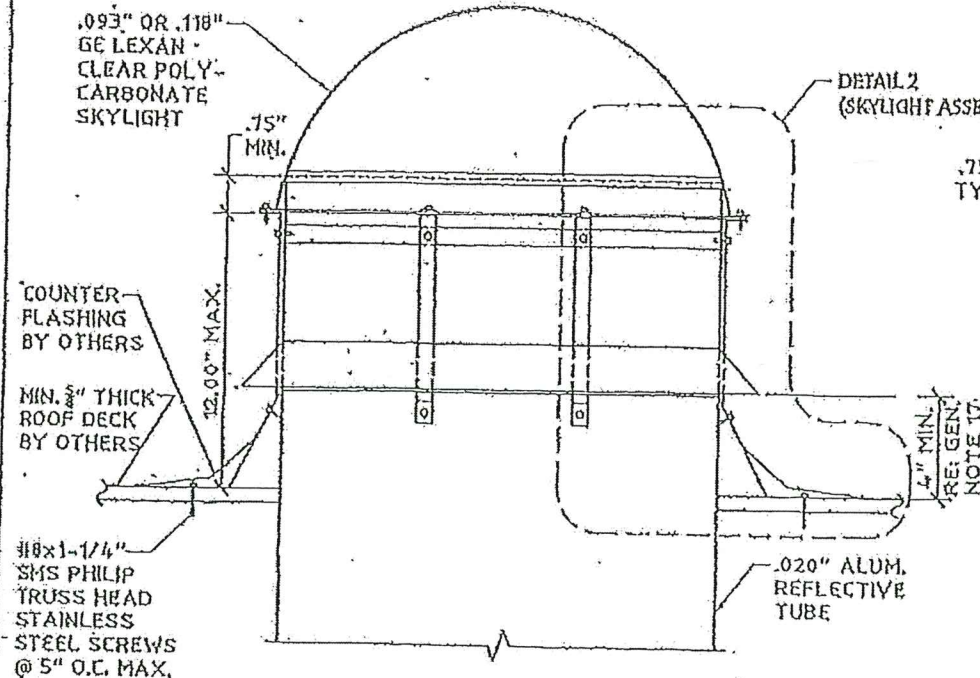
① STANDARD FLAT ROOF MOUNT (STD-F MODEL) SCALE: 1-1/2" = 1' - 0"
