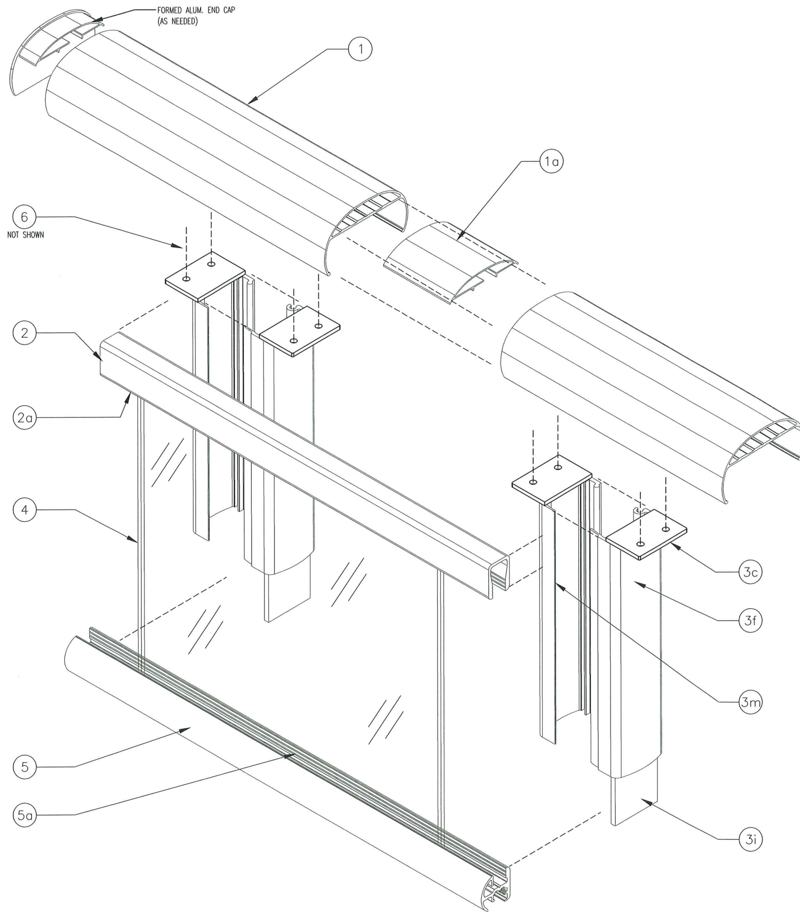
EMBEDDED POST GUARDRAIL ASSEMBLY EXPLODED VIEW
