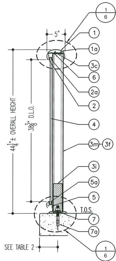
RAILING PROFILE NTS
