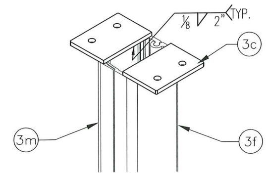
PIVOTING POST IN FIXED POSITION
