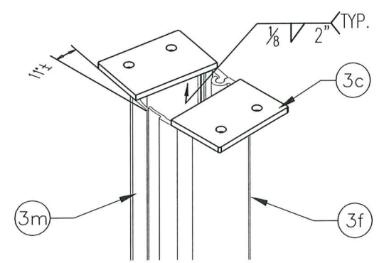
PIVOTING POST IN ROTATION
