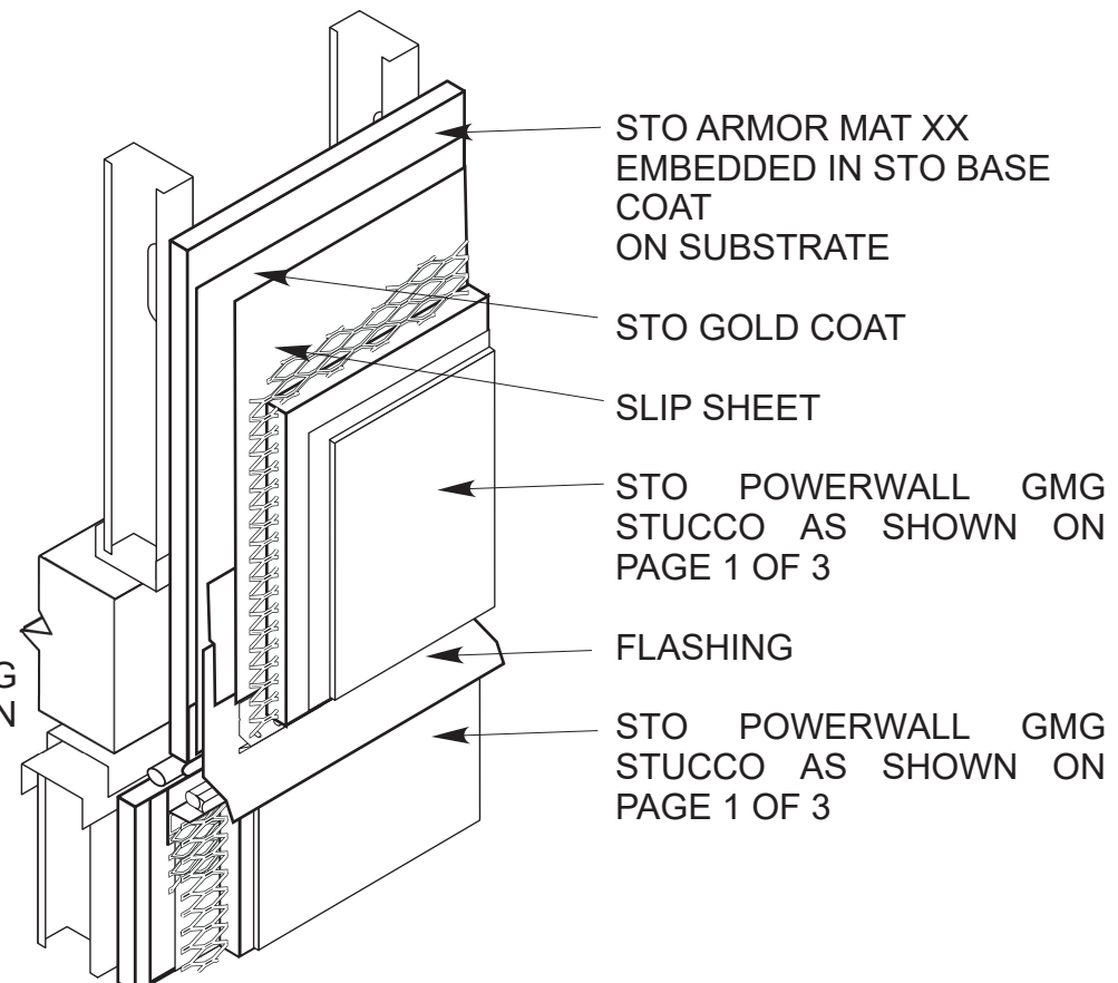
FLOOR LINE JOINT WITH FLASHING
