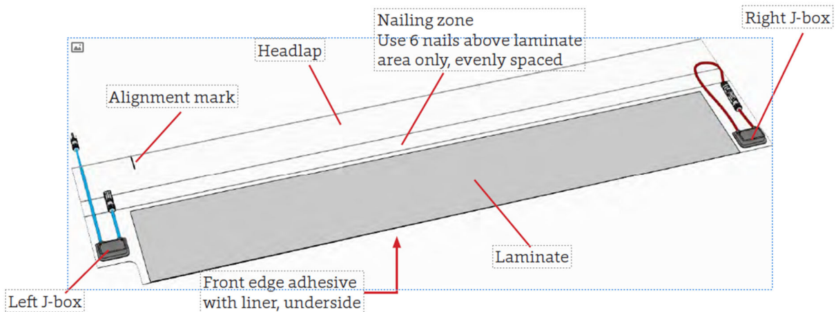
Figure 8. Jumper module (JM)
