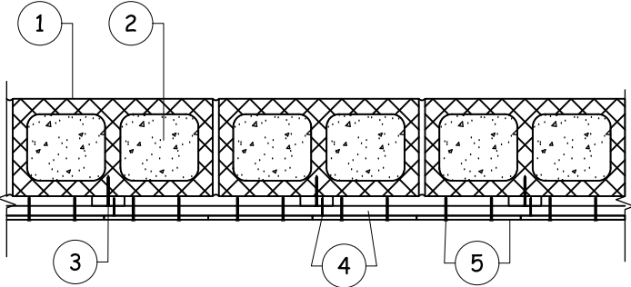
A 5 HANDSPPLIT SHAKES OVER GROUTED CMU WALL PLAN VIEW NOT-TO-SCALE
