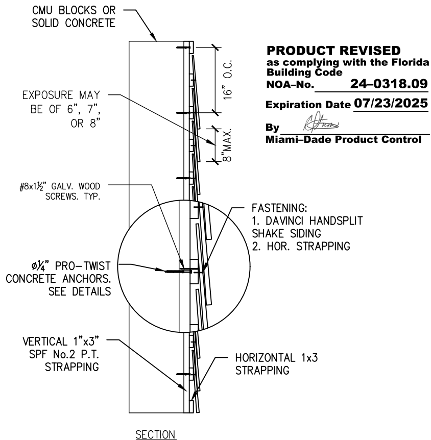
INSTALLATION - SECTION
