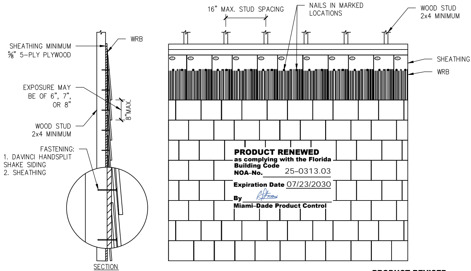
A 1 INSTALLATION – SECTION B 1 INSTALLATION ELEVATION
