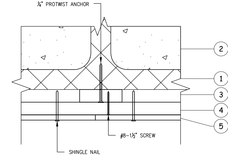
B 5 HANDSPPLIT SHAKES OVER GROUTED CMU WALL PLAN VIEW NOT-TO-SCALE
