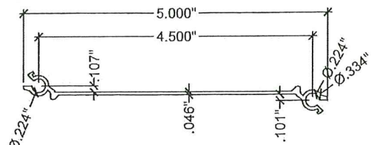
(G1) MALE/MALE SOLID BLADE SPA002-MM
