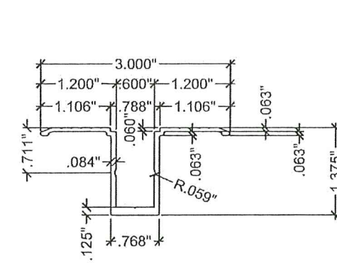
(D1) FLOOR SILL SPA012
