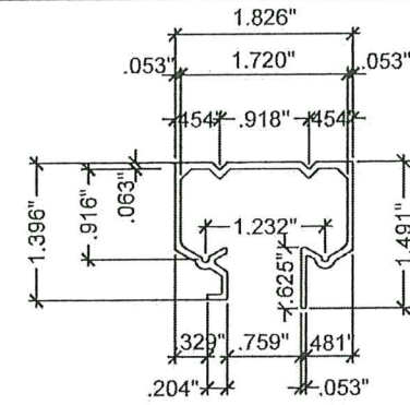
(A1) CEILING HEADER (& INVERTED) LIGHT DUTY SPA016
