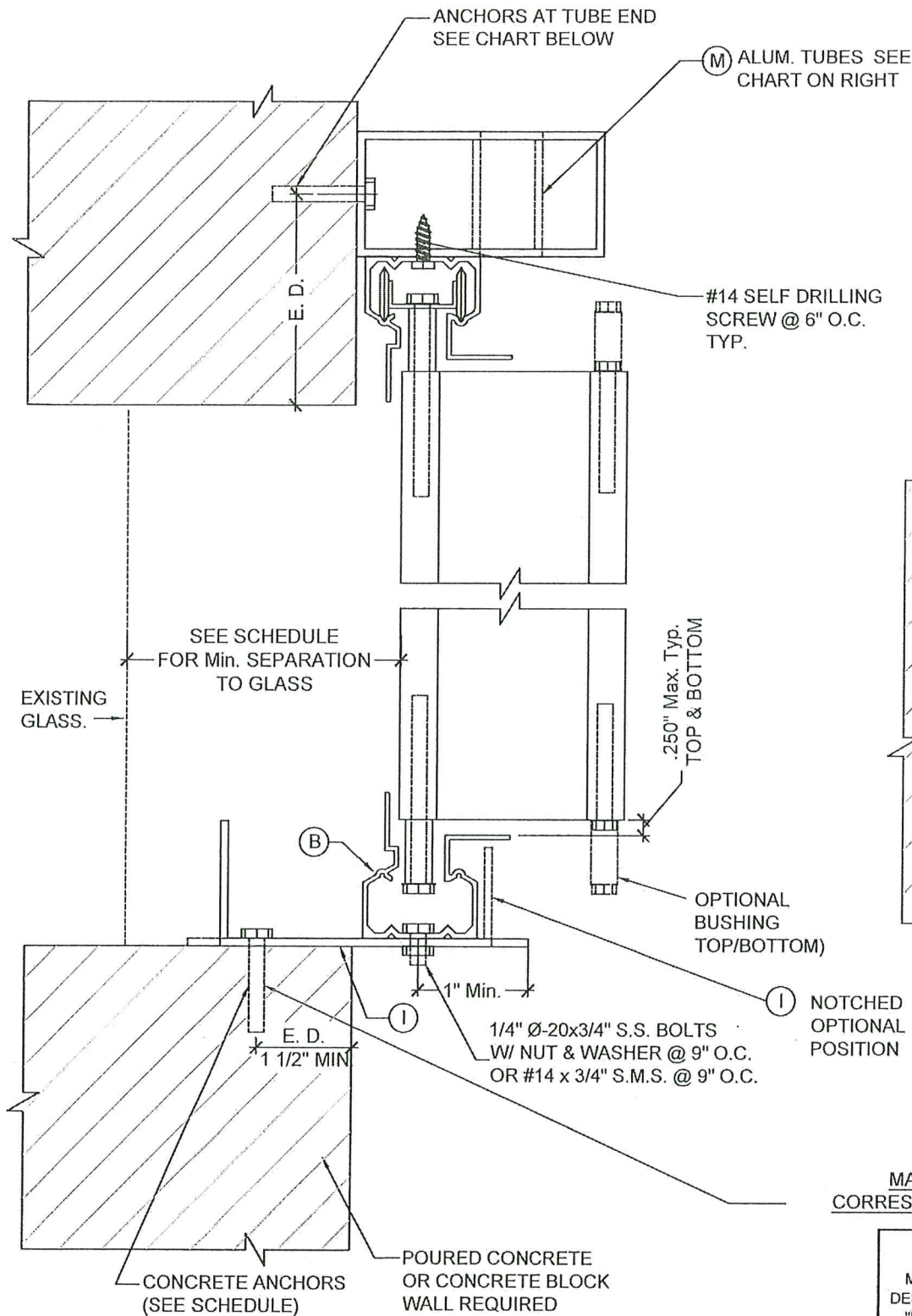
BUILD-OUT INSTALLATION SECTION M
