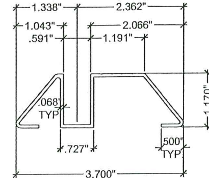
(D2) THRESHOLD TRACK SPA011
