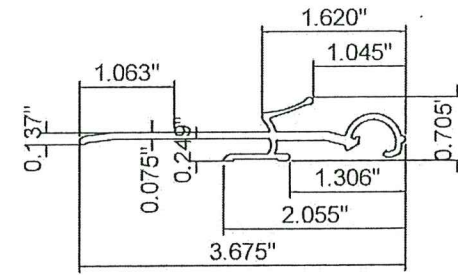
(HL) CENTER MATE LIGHT DUTY SPA017
