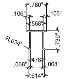
(N) SNAP COVER SPA013
