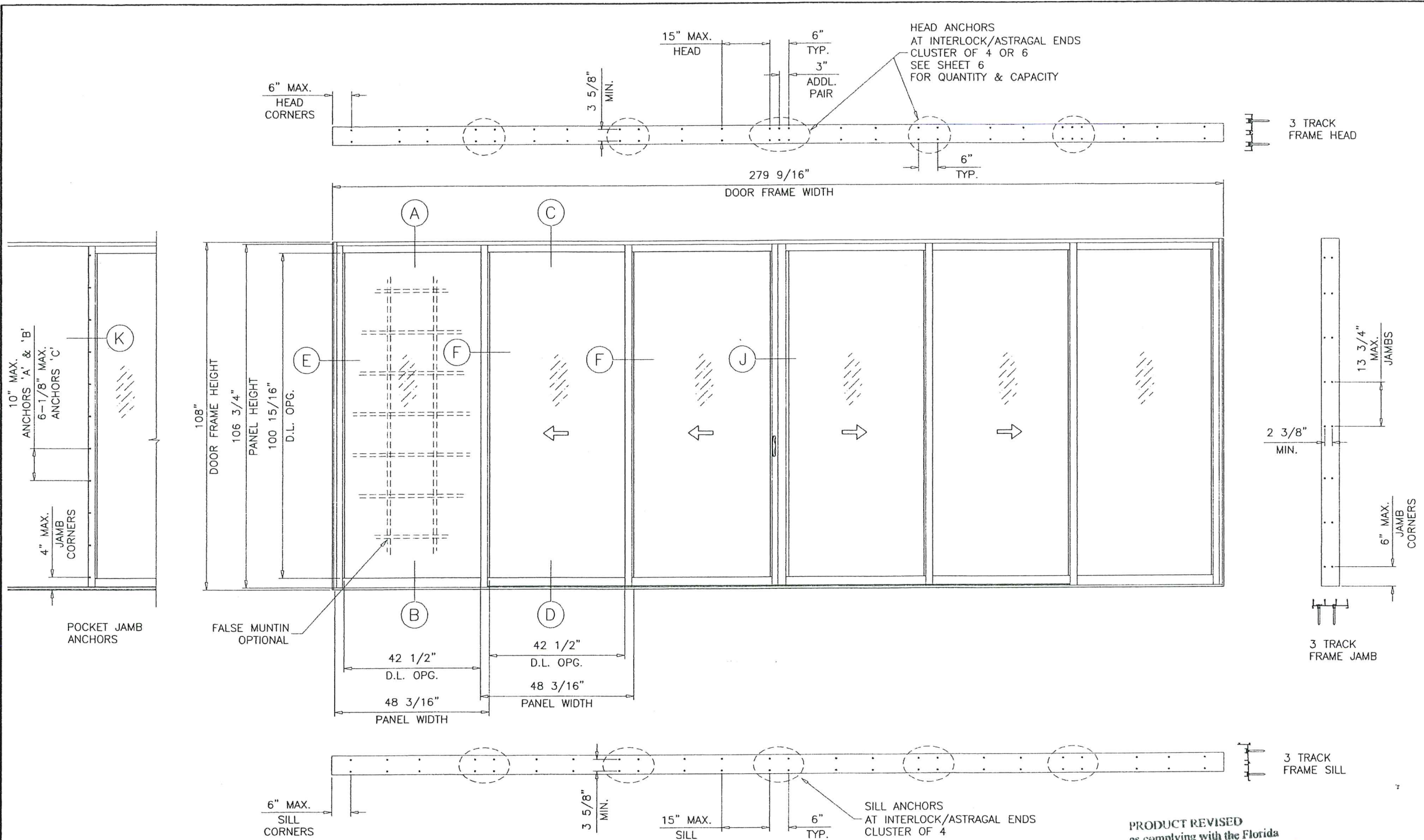
TYPICAL ELEVATION OXX-XXO
