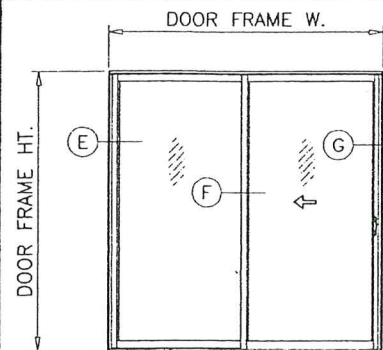
OX (SHOWN) XO
