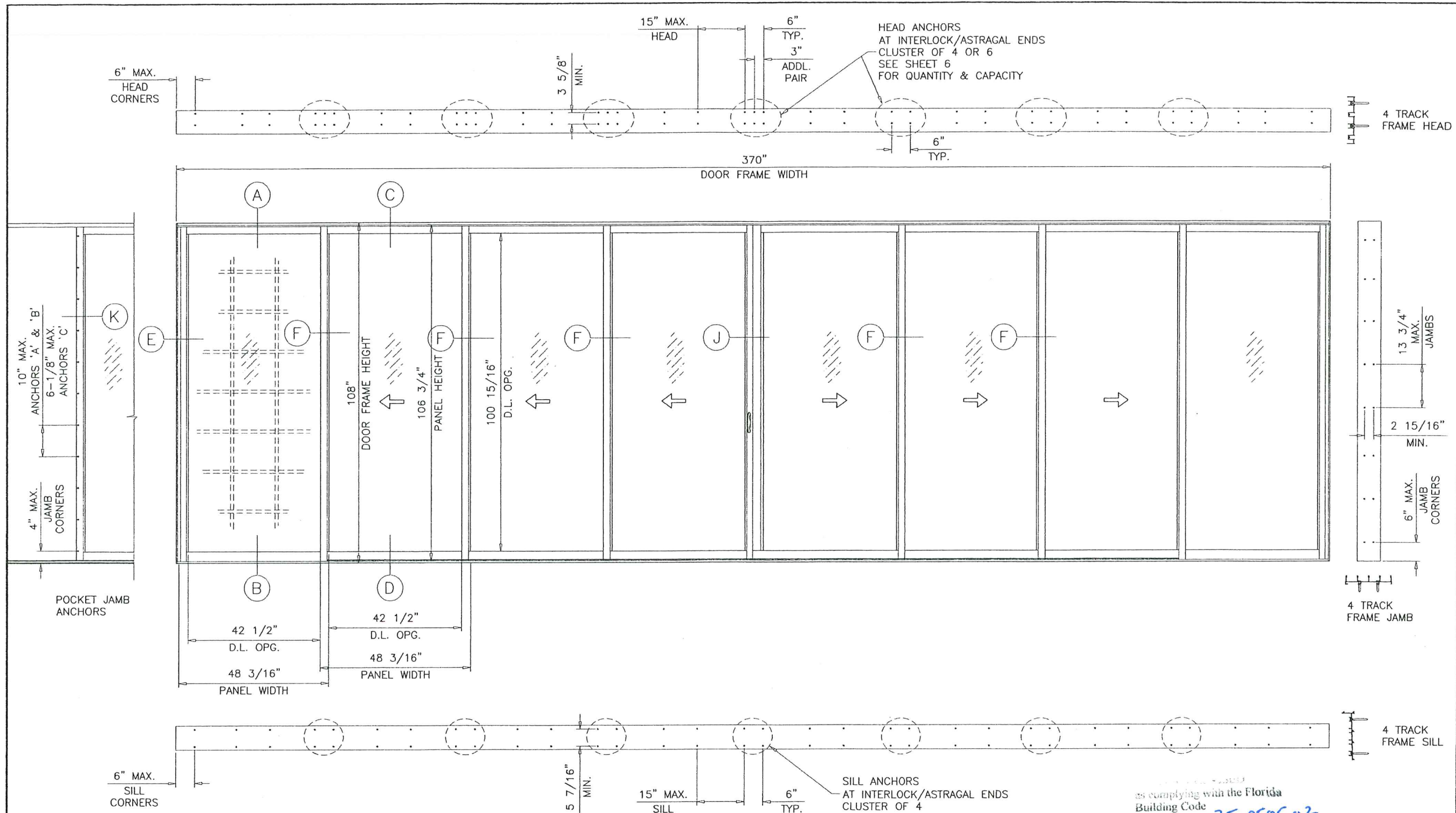
TYPICAL ELEVATION OXXX-XXXX
