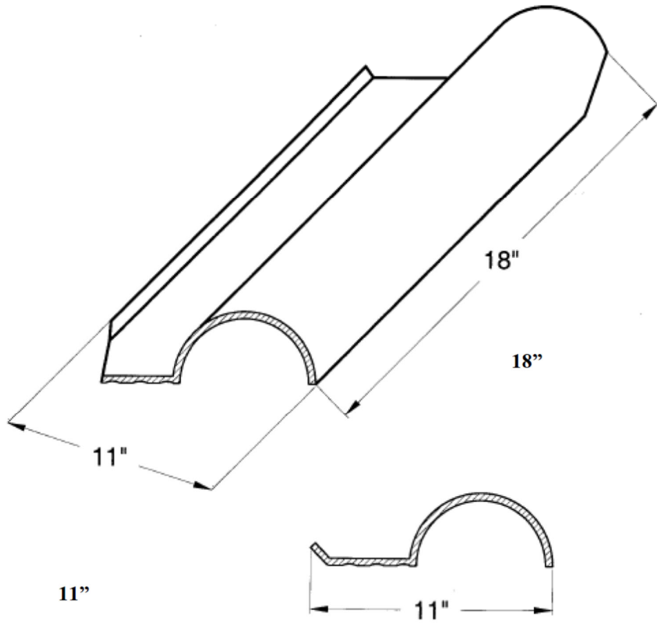
BARRANQUILLA SPANISH 'S' CLAY ROOF TILE
