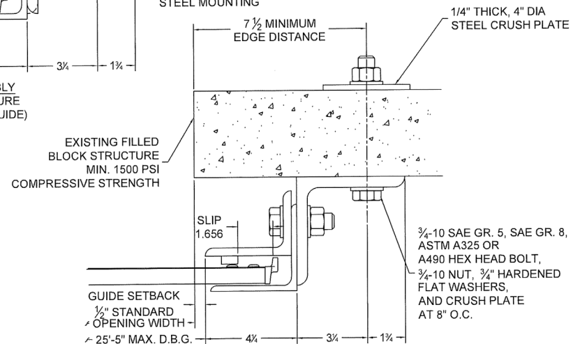
⑪ GUIDE ASSEMBLY FILLED BLOCK STRUCTURE (Z-GUIDE)
