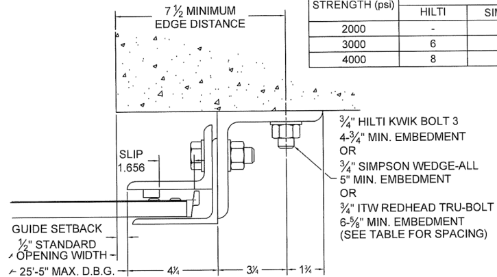
⑧ GUIDE ASSEMBLY CONCRETE STRUCTURE (Z-GUIDE)
