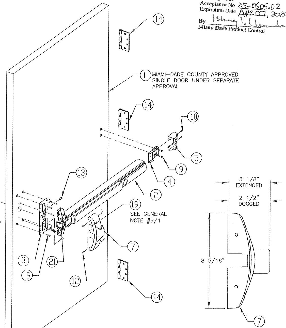
ASSEMBLY (ISOMETRIC) N.T.S. WIDE STILE 10 SERIES SHOWN
