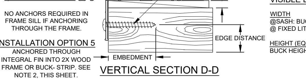
VERTICAL SECTION D-D
