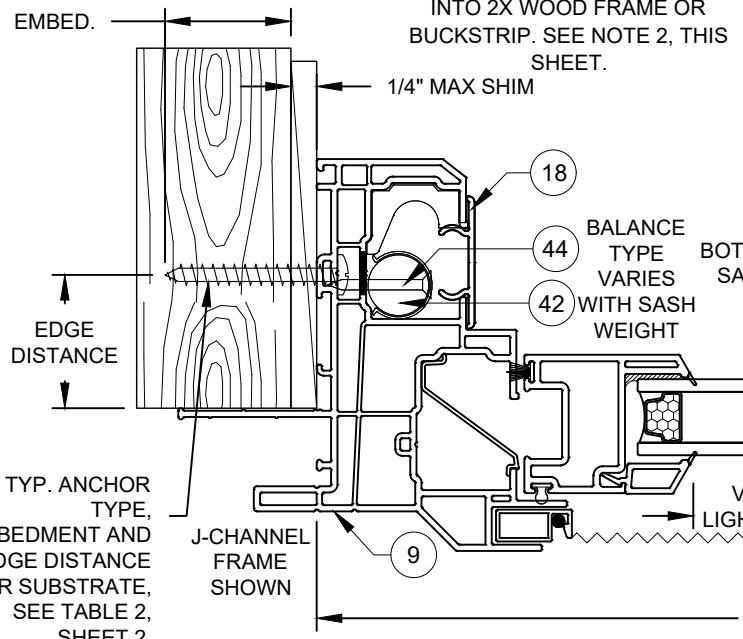
HORIZONTAL SECTION C-C
