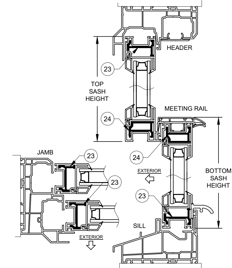
SECTION DETAIL FOR WINDOWS WITH LEVEL R1 REINFORCEMENT & GLASS TYPES 1-4 (REINFORCEMENTS SHOWN IN FIGURES ABOVE APPLY TO ALL FRAME TYPES & CONFIGURATIONS)
