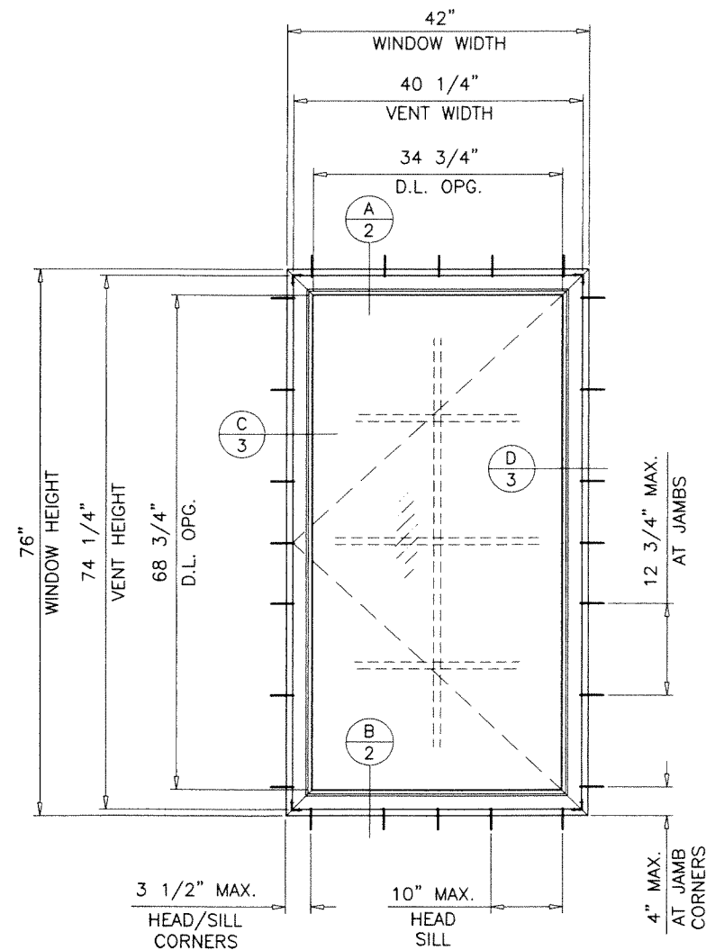
TYPICAL ELEVATION
