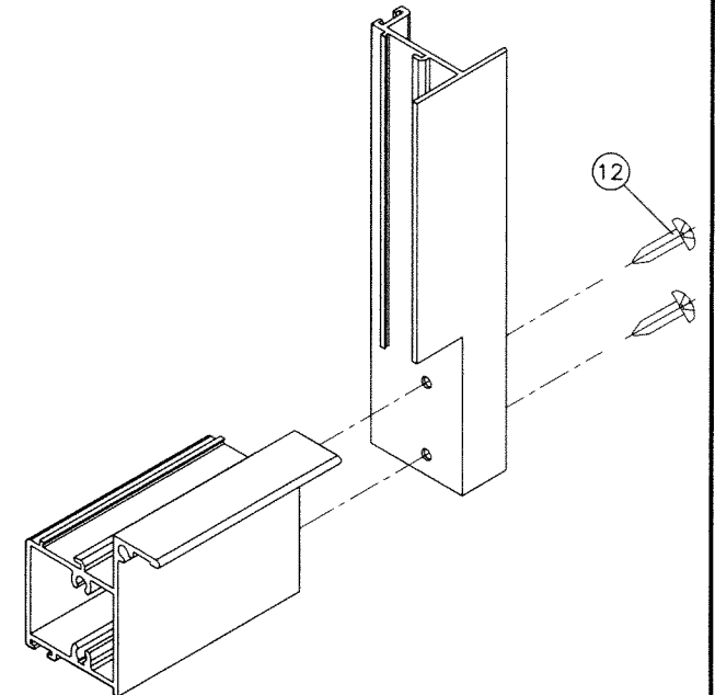
VENT CORNER DETAIL
