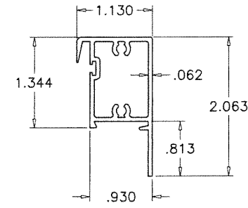
⑤B STD. VENT TOP RAIL SERIES-1050
