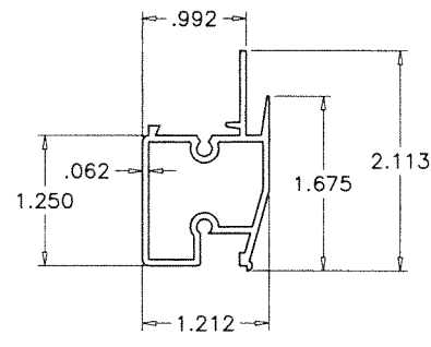
④ MEETING RAIL SERIES-1000
