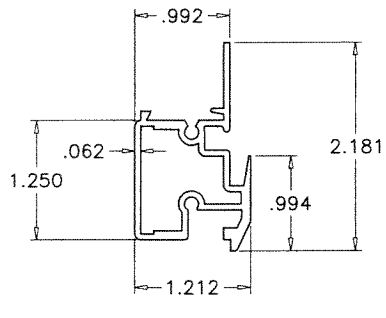
④A MEETING RAIL SERIES-1050
