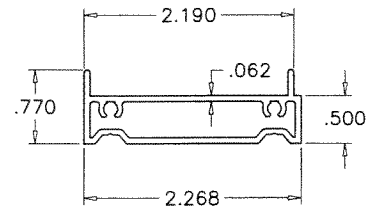
⑱ FLUSH FRAME ADAPTER
