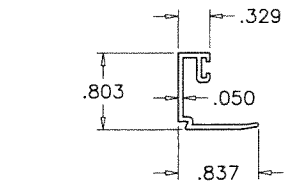
⑧A SQUARE GLAZING STOP
