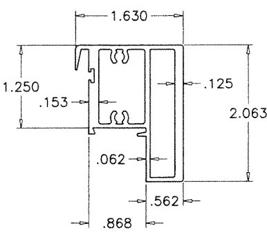
⑤C.1 H.D. VENT TOP RAIL SERIES-1050
