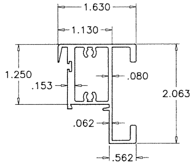
⑤C H.D. VENT TOP RAIL SERIES-1050
