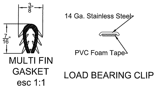
DW4000 PANEL JOINT DETAIL AT SUPPORTS ①
