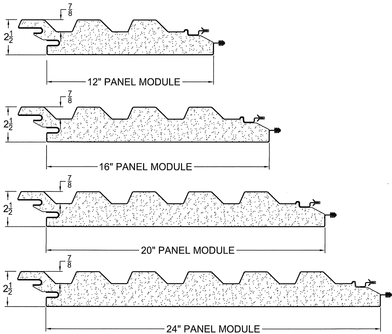
DESIGNWALL 2000R INSULATED METAL PANEL
