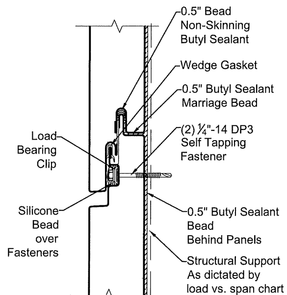
DW4000 PANEL JOINT DETAIL AT SUPPORTS AT END OF PANEL ②
