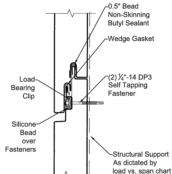
DW4000 PANEL JOINT DETAIL AT SUPPORTS ①
