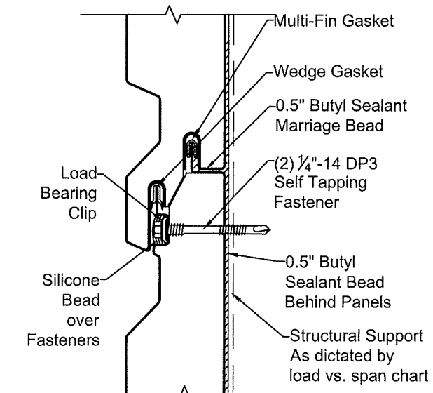
DW2000R & DW2000R-459 PANELS JOINT DETAIL AT SUPPORTS AT END OF PANEL ②
