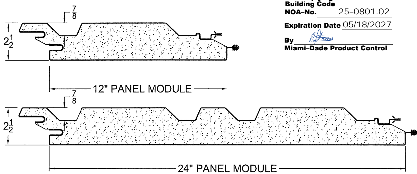
DESIGNWALL 2000R-459 INSULATED METAL PANEL
