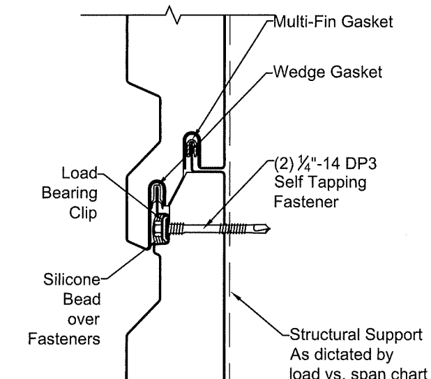
DW2000R & DW2000R-459 PANELS JOINT DETAIL AT SUPPORTS ①
