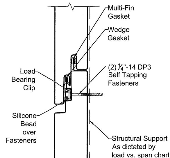
DW2000 PANEL JOINT DETAIL AT SUPPORTS ①
