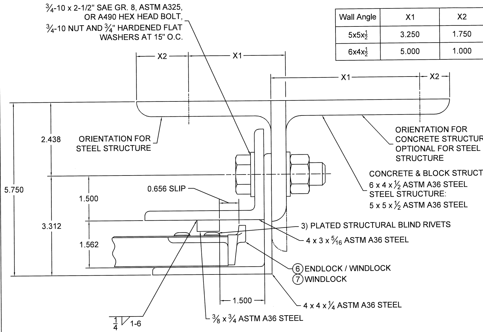
② GUIDE ASSEMBLY DETAIL 1:2 SCALE
