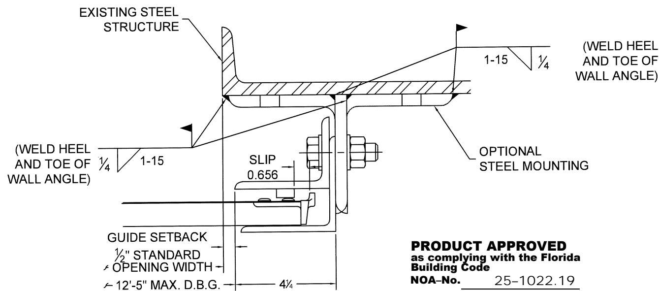
⑬ GUIDE ASSEMBLY STEEL STRUCTURE (Z-GUIDE OR E-GUIDE)
