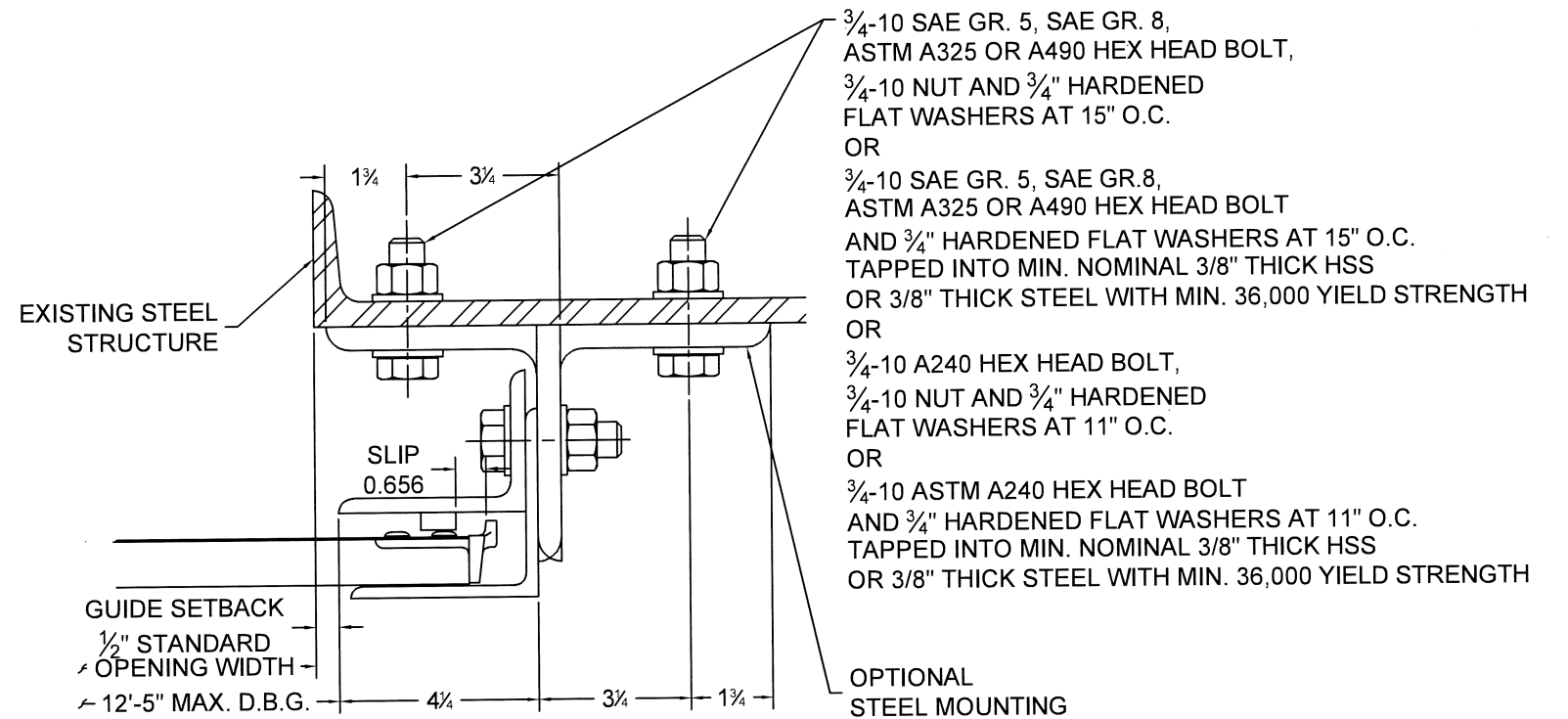
⑭ GUIDE ASSEMBLY STEEL STRUCTURE (Z-GUIDE OR E-GUIDE)
