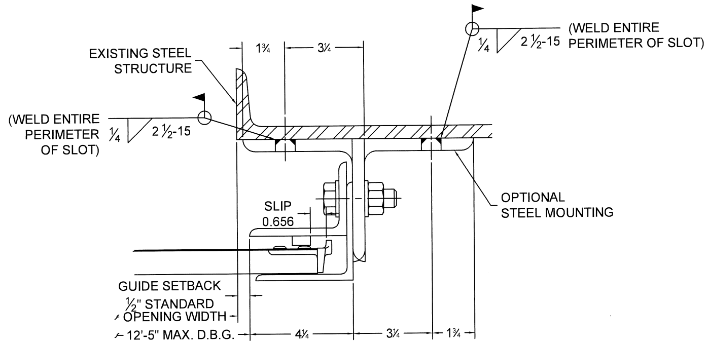
⑫ GUIDE ASSEMBLY STEEL STRUCTURE (Z-GUIDE OR E-GUIDE)
