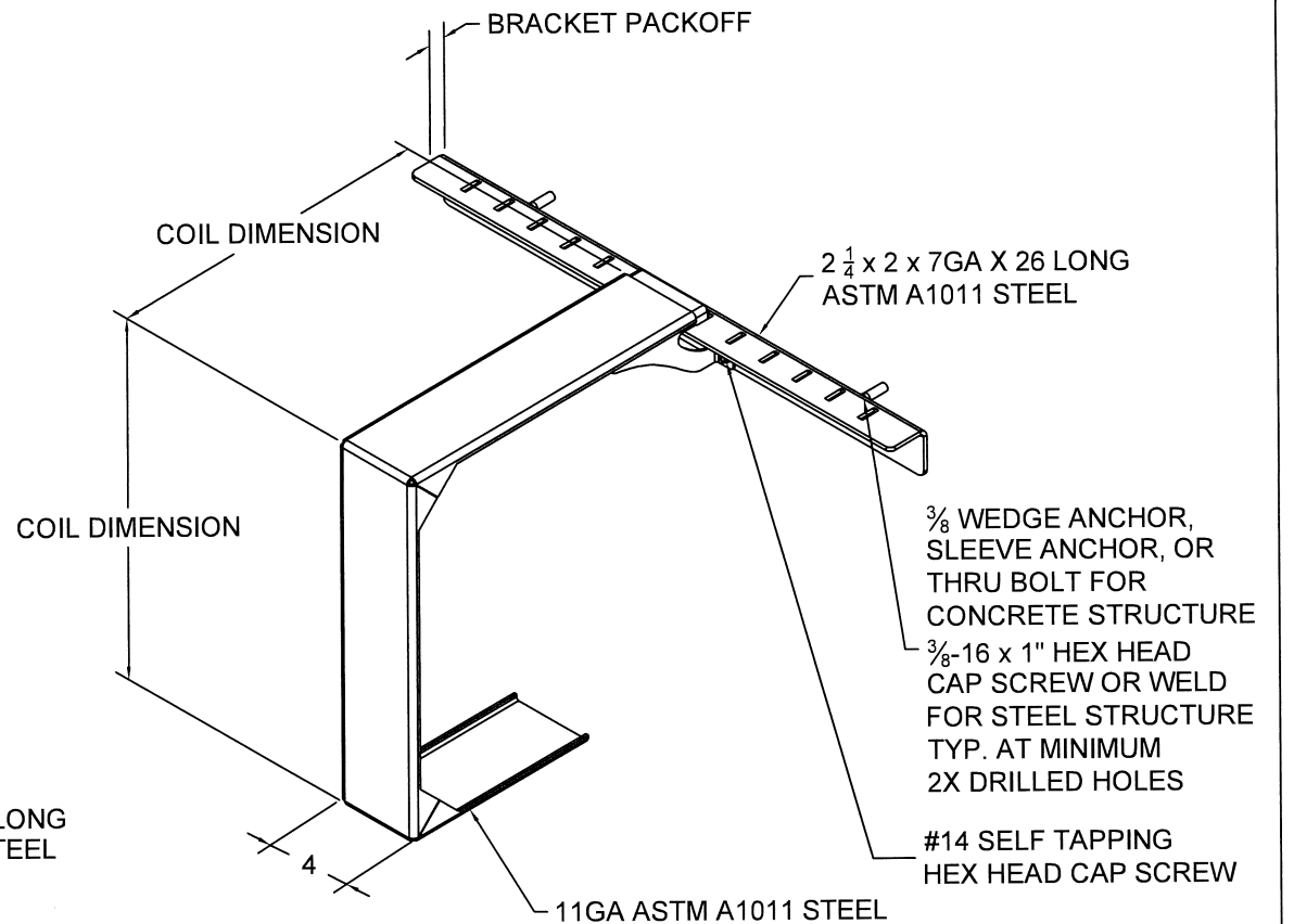
⑱ MID-HOOD SUPPORT (WHEN REQUIRED) SQUARE STYLE DEPICTED, "D" SHAPE ALSO AVAILABLE SCALE: NTS
