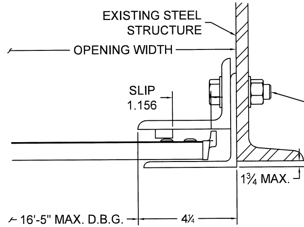
⑮ GUIDE ASSEMBLY STEEL STRUCTURE (BETWEEN JAMBS GUIDE)
