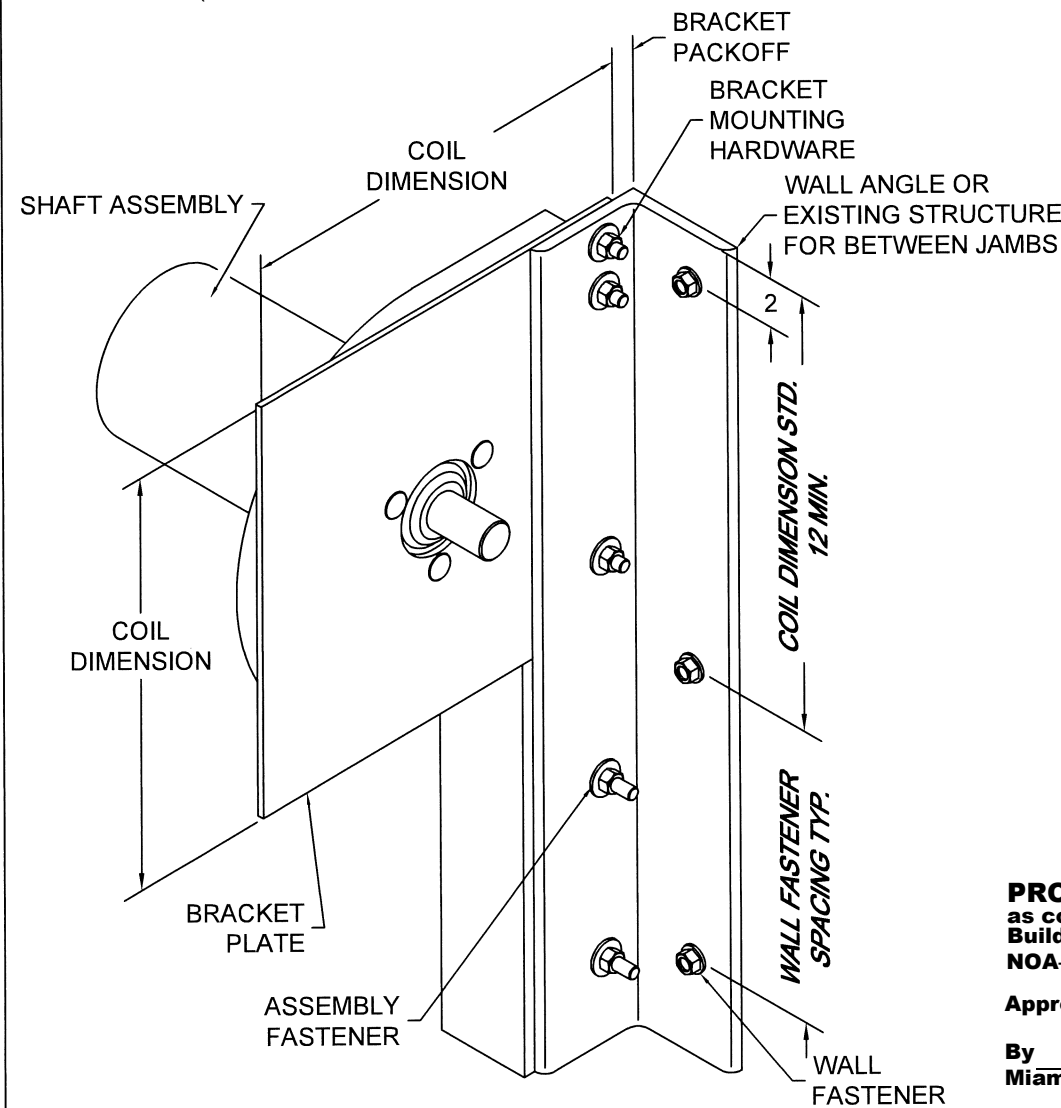
⑯ BRACKET MOUNTING / TOP WALL ANGLE FASTENING BRACKET MOUNTING PER DETAIL 8 DEPICTED, OTHER BRACKET MOUNTINGS ARE AVAILABLE SCALE: NTS
