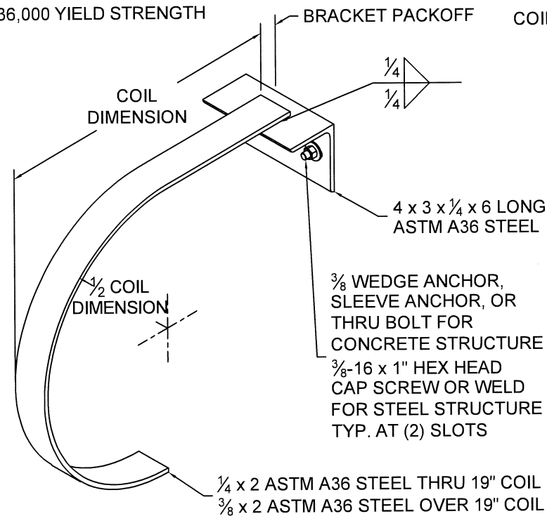
⑰ MID-HOOD SUPPORT (WHEN REQUIRED) "D" SHAPE DEPICTED, SQUARE STYLE ALSO AVAILABLE SCALE: NTS
