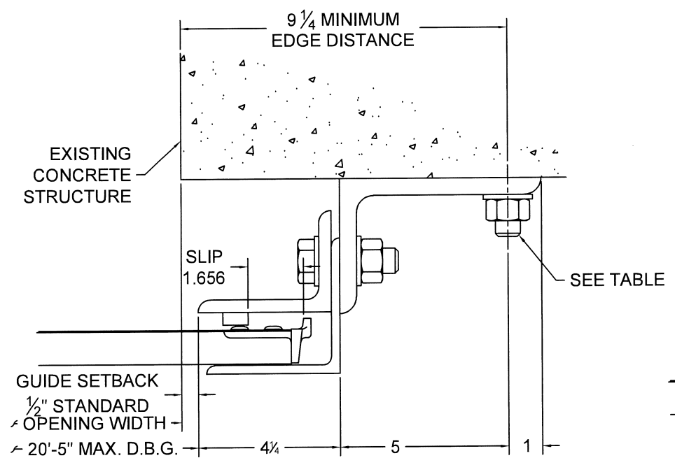
(9) GUIDE ASSEMBLY CONCRETE STRUCTURE (Z-GUIDE)
