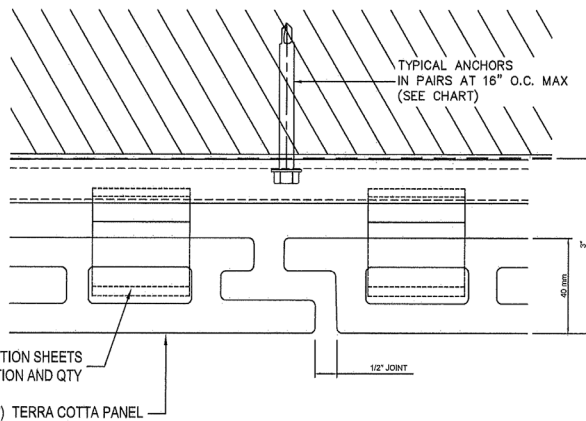
K VERTICAL PANEL / PANEL SCALE: .5 = 1.0
