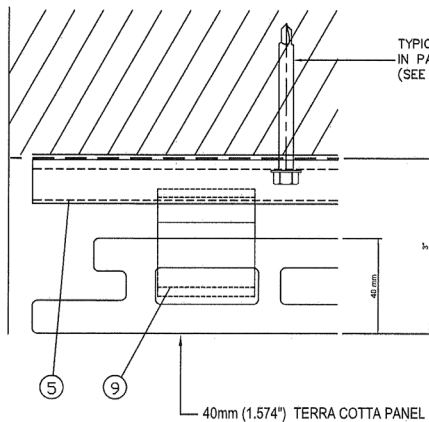
J PANEL JAMB SCALE: .5 = 1.0
