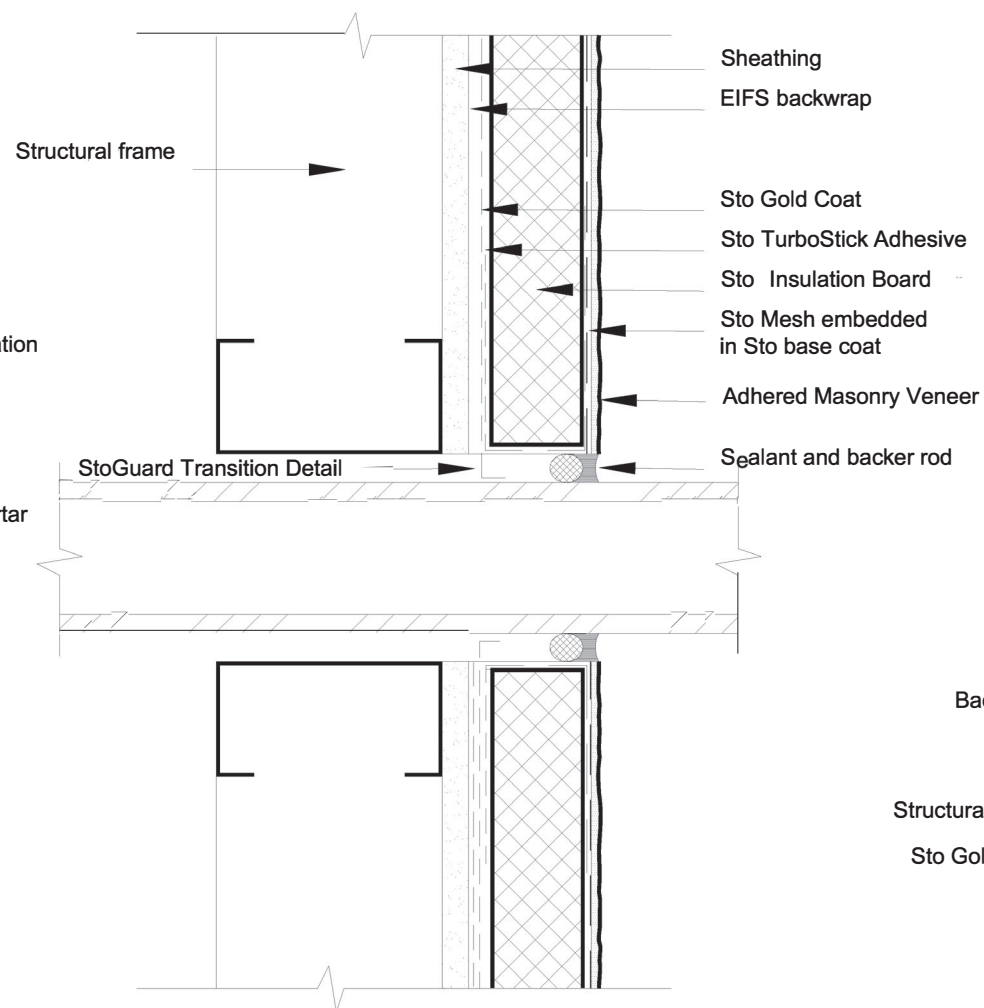
TERMINATION AT PENETRATION N.T.S.
