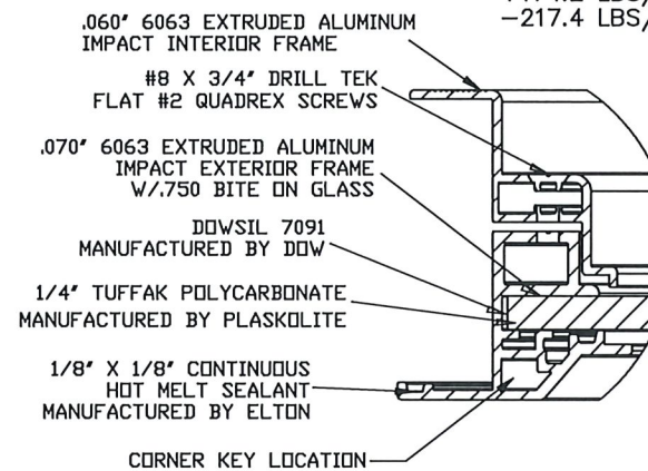
EXPANDED IMPACT WINDOW DETAIL N.T.S.
