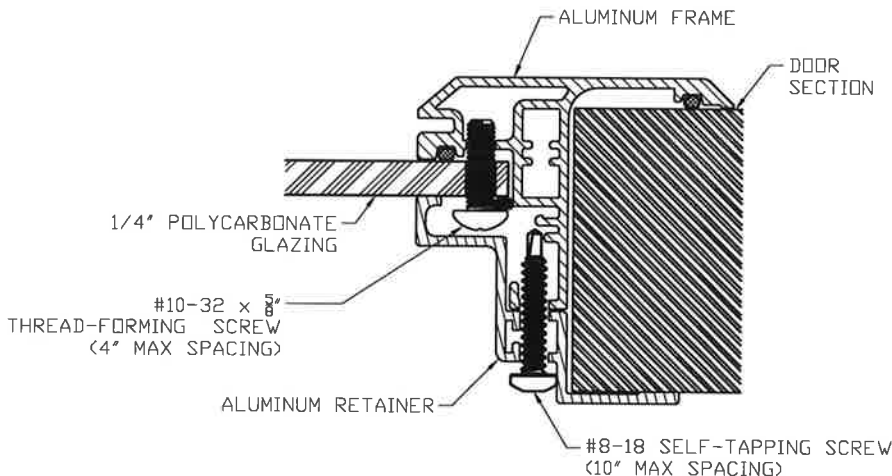
IMPACT-RESISTANT GLAZING DETAILS
