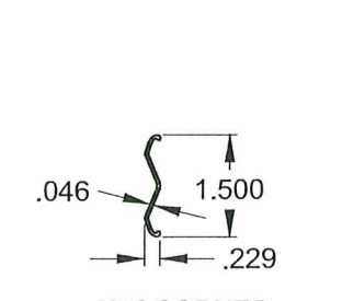
㊳ 135° CORNER ASTRAGAL CAP, INTERIOR
