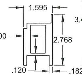
㉘ INTERLOCK .400 REINFORCEMENT, HEAVY-DUTY
