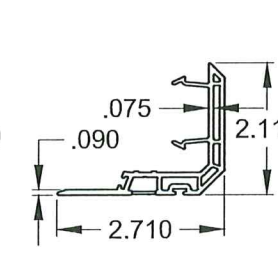
㉛ INTERLOCK ADAPTER
