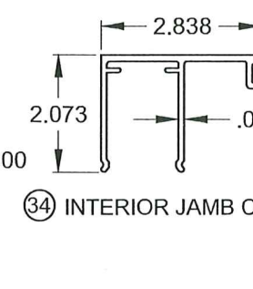
㉞ INTERIOR JAMB COVER
