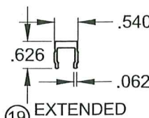
⑲ EXTENDED KEEPER
