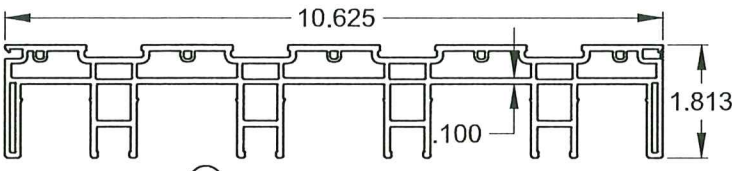
⑤ 4 TRACK HEAD/JAMB
