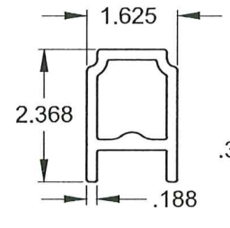
㉖ TOP, BOTTOM AND STILE COMPOSITE REINFORCEMENT
