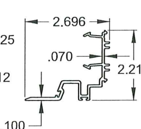
㉚ EXTENDED POCKET INTERLOCK ADAPTER
