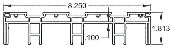
③ 3 TRACK HEAD/JAMB
