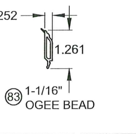
㊵ 1-1/16" OGEE BEAD
