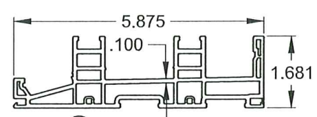
② 2 TRACK SILL
