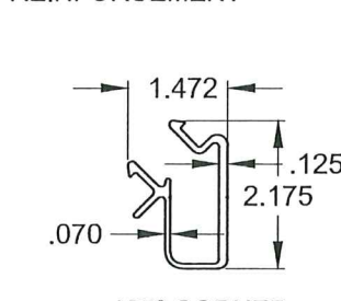
㊱ 135° CORNER PASSIVE MOUNT
