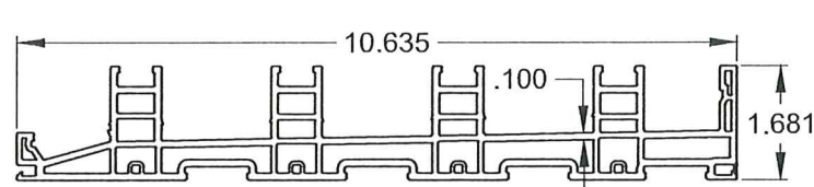
⑥ 4 TRACK SILL
