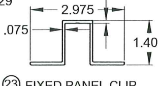
㉓ FIXED PANEL CLIP
