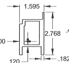
㉗ INTERLOCK .300 REINFORCEMENT, STANDARD
