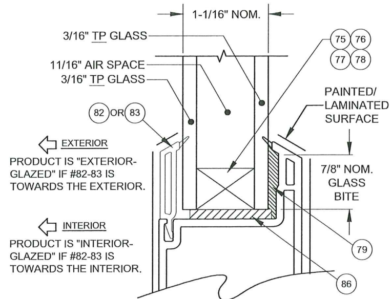
GLASS DETAIL
