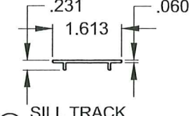
⑬ SILL TRACK COVER
