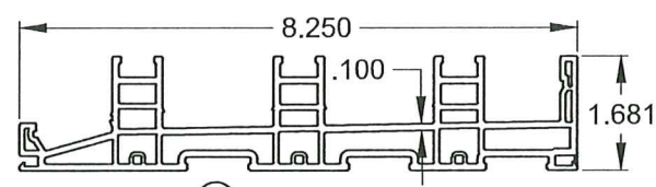
④ 3 TRACK SILL
