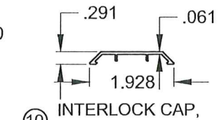
⑩ INTERLOCK CAP, EXTENDED POCKET
