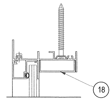
ALTERNATE DETAIL WITH FASTENER COVER
