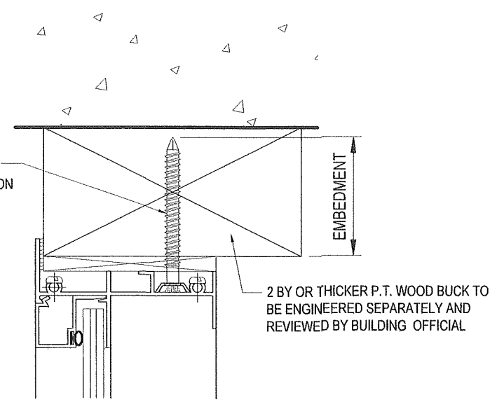
ANCHORAGE OPTION INTO WOOD
