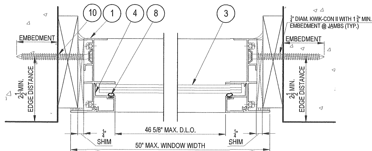
3A UNEQUAL LEG CONDITION 4A
