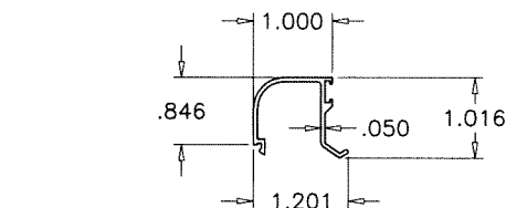
4 GLAZING BEAD
