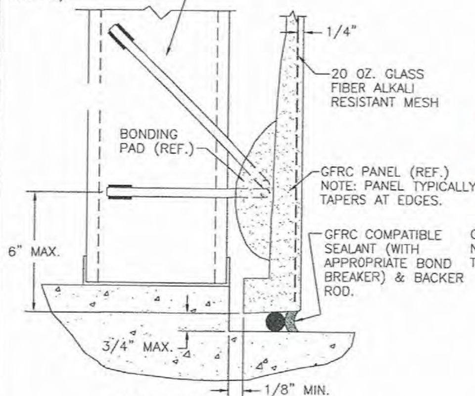
WALL BASE DETAIL
