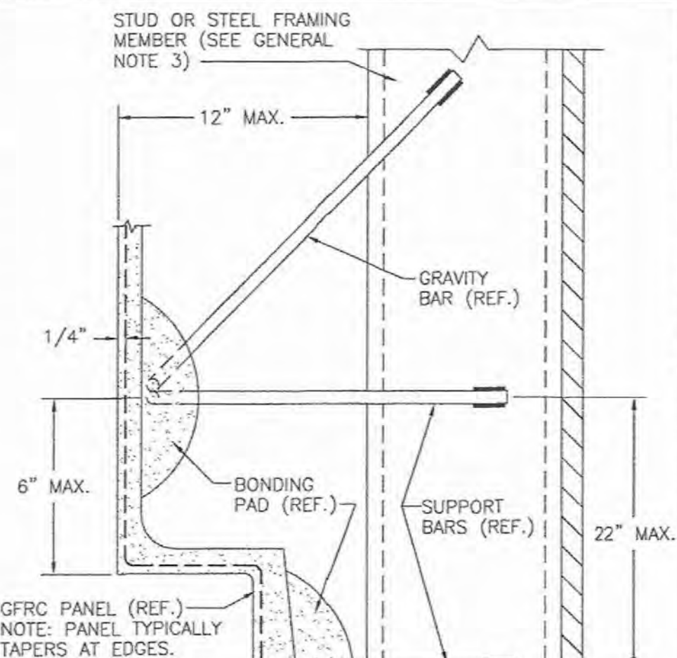
TYP. WINDOW/DOOR HEAD DETAIL
