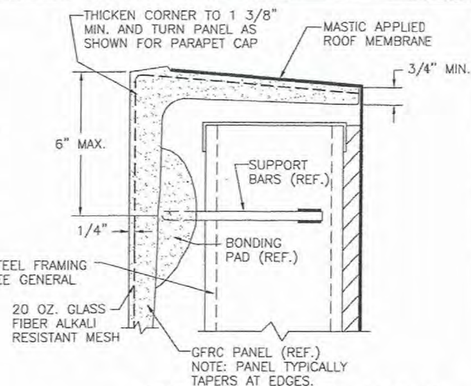
PARAPET DETAIL WITHOUT FLASHING
