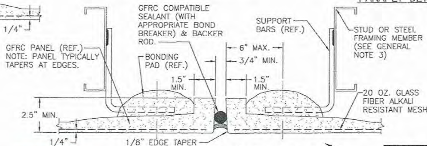
OPTIONAL CONTROL/EXPANSION JOINT
