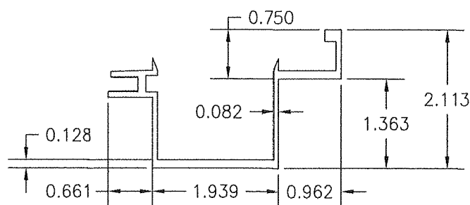
EXTRUDED ALUMINUM CHANNEL
