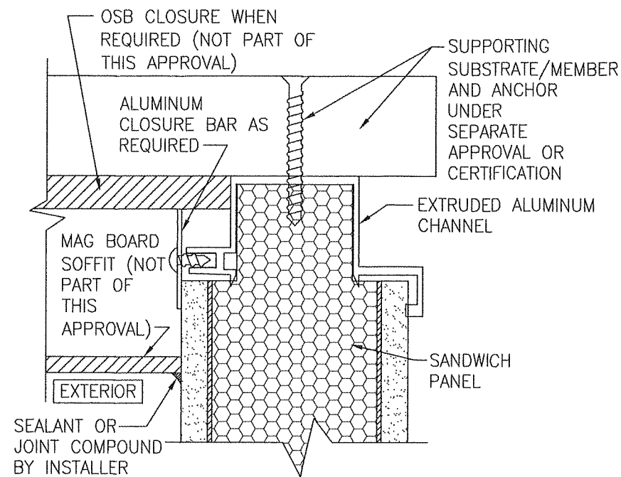
TYPICAL DETAIL AT TOP OF WALL
