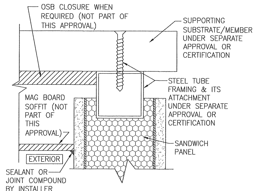
TYPICAL ALTERNATE DETAIL AT TOP OF WALL
