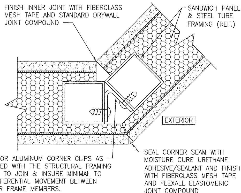
45 DEG. OUTER CORNER DETAIL
