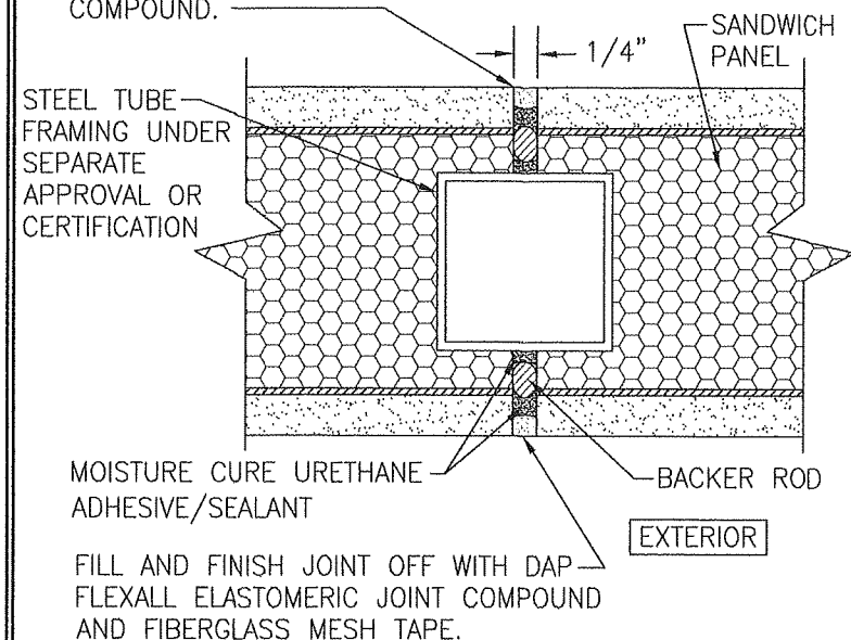
TYPICAL DETAIL AT INTERMEDIATE SUPPORT FRAMING (HORIZONTAL & VERTICAL JOINTS)
