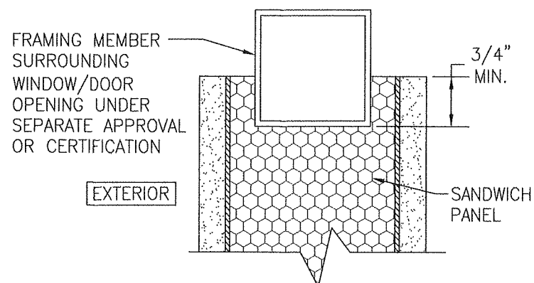
TYPICAL DETAIL AT WINDOW/DOOR OPENING
