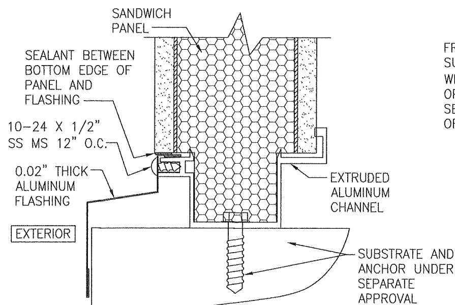
TYPICAL DETAIL AT BASE OF WALL
