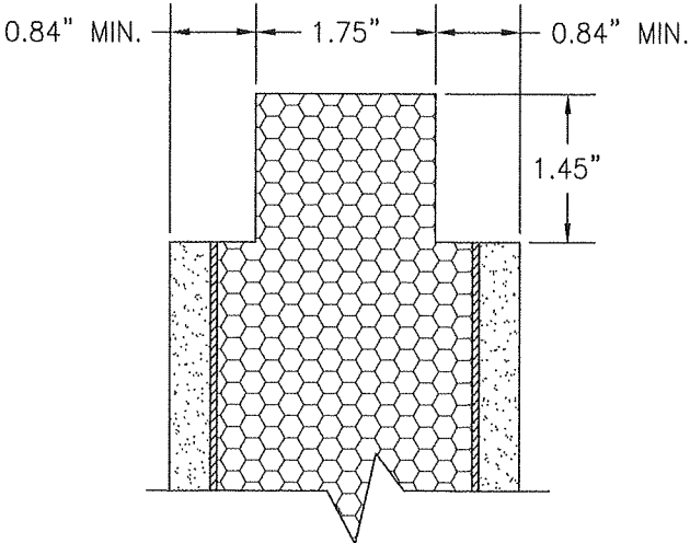
SECTION B SCALE: 1/2 FULL (FOR ALL PANEL DIMENSIONING & INFORMATION NOT SHOWN, SEE SECTION A/1)
