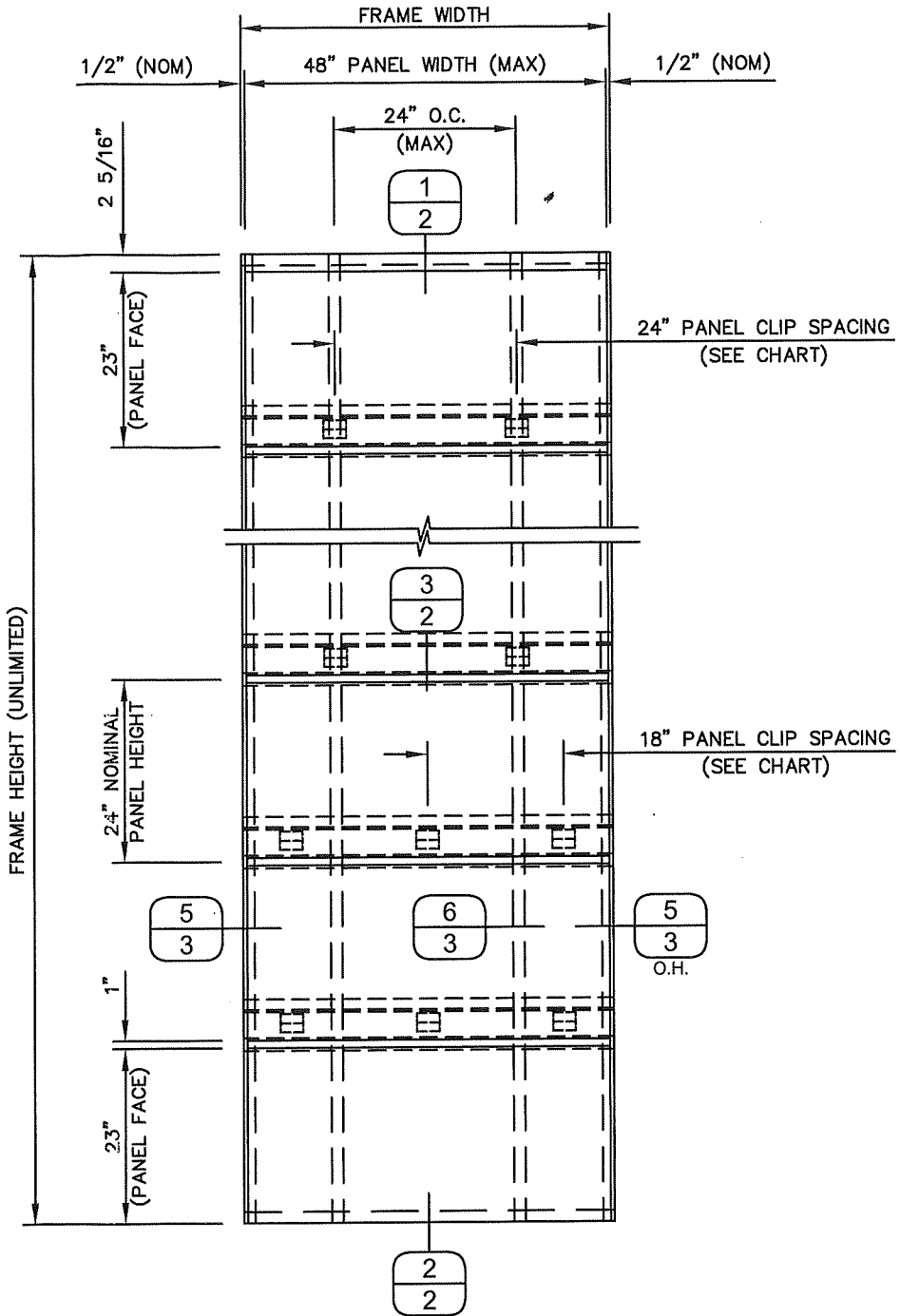
EXTERIOR VIEW (NOT TO SCALE)
