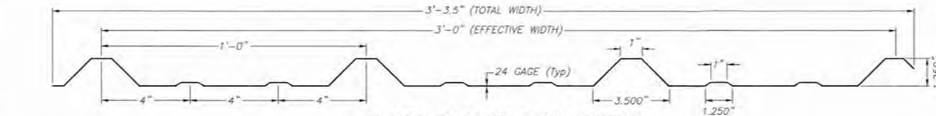
FLORIDA RIB PANEL CROSS SECTION
