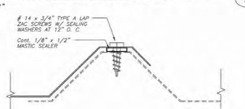
TYPICAL ROOF PANEL SIDE LAP DETAIL (SECTION)
