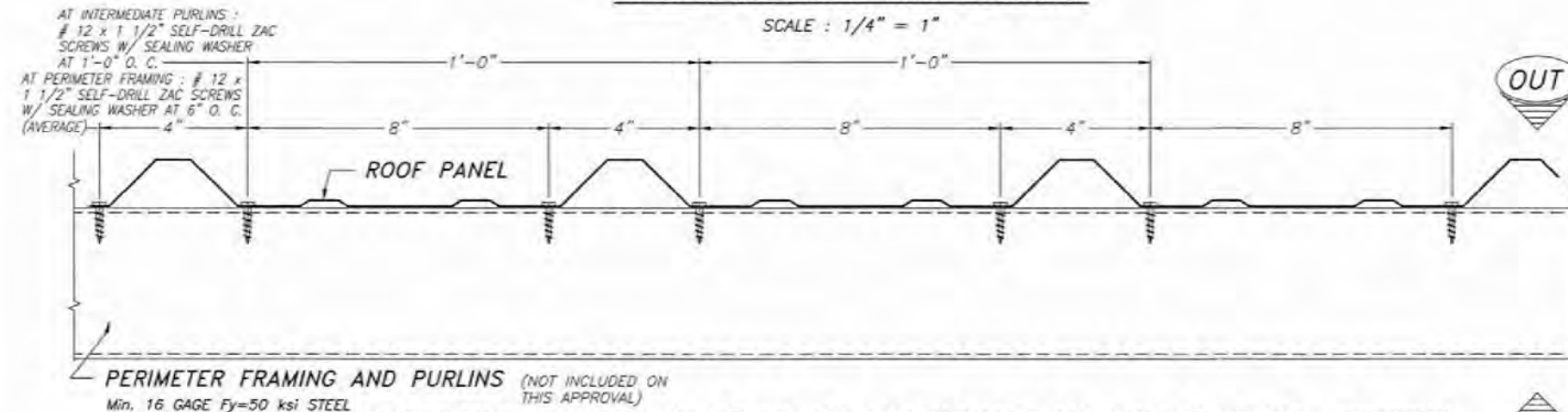
TYPICAL ROOF PANEL CONNECTION DETAIL TO INTERMEDIATE AND END SUPPORT (SECTION)
