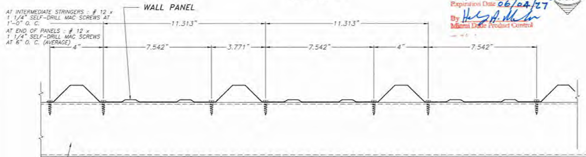
TYPICAL WALL PANEL CONNECTION DETAIL TO INTERMEDIATE AND END SUPPORT (SECTION)
