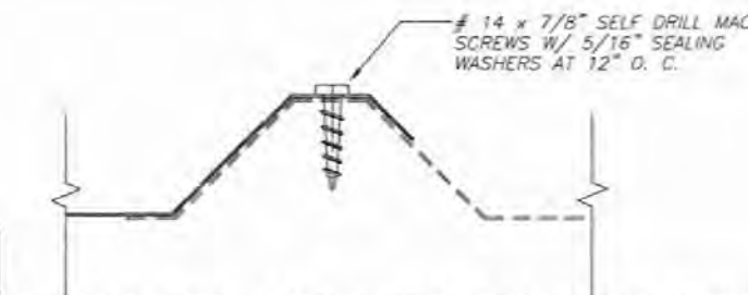
TYPICAL WALL PANEL SIDE LAP DETAIL (SECTION)
