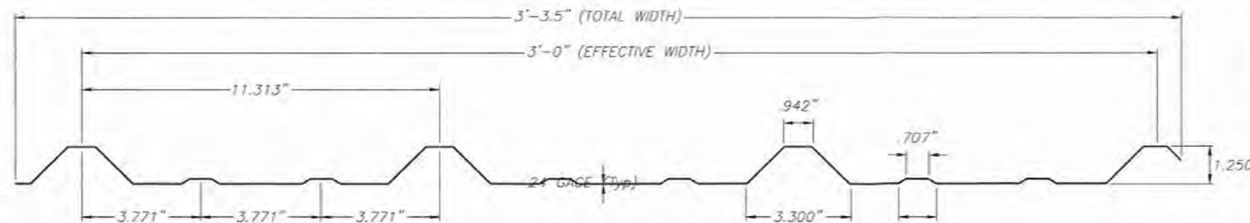
FLORIDA RIB PANEL CROSS SECTION
