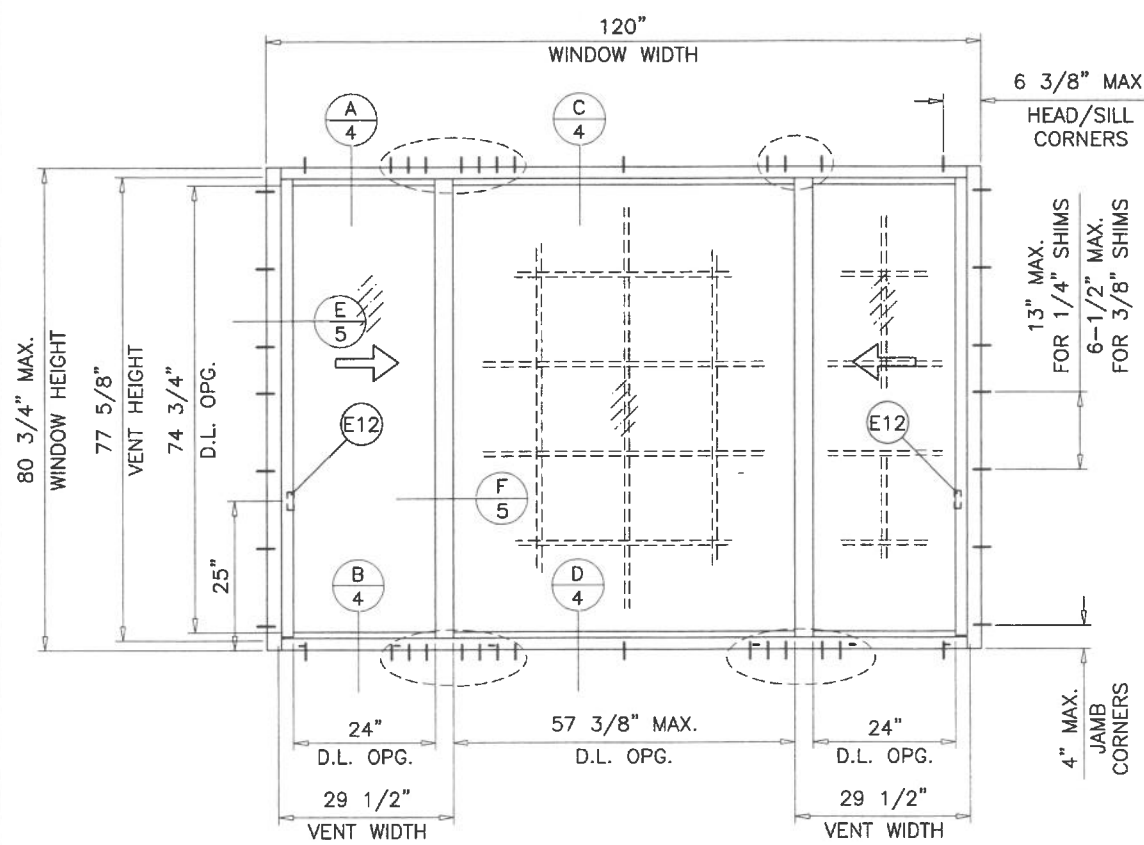
TYPICAL ELEVATIONS
