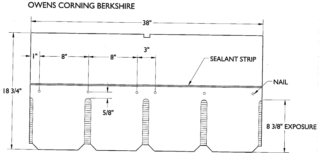
FASTENING PATTERN & PHYSICAL DIMENSIONS
