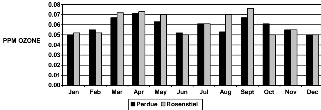
Figure 3. Eight-Hour Maximum Monthly Ozone Concentrations – 2005
