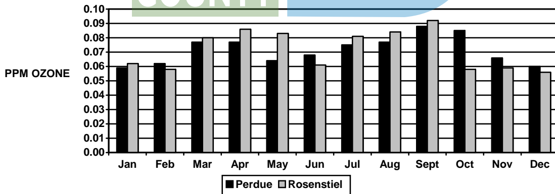
Figure 2. One-Hour Maximum Monthly Ozone Concentrations – 2005
