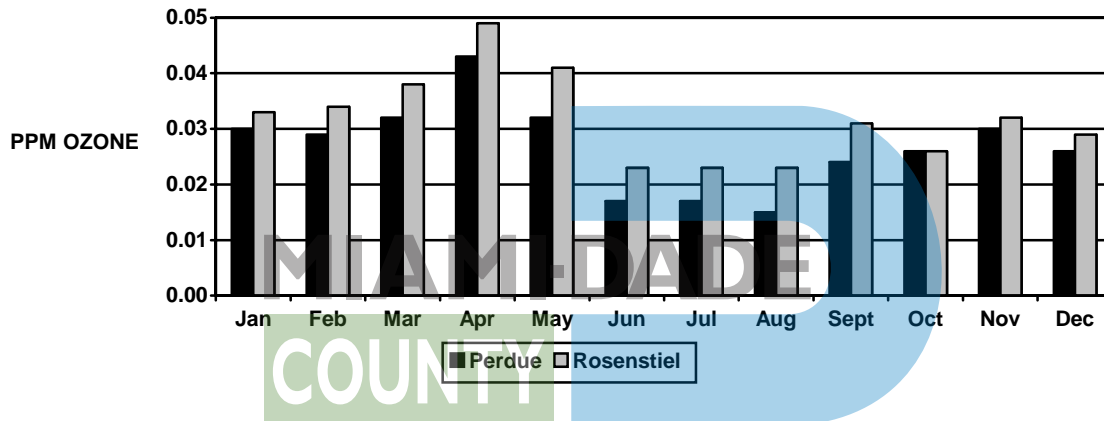
Figure 4. Average Monthly Ozone Concentrations – 2005
