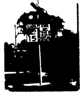
Solar powered school speed zone flashing signal
