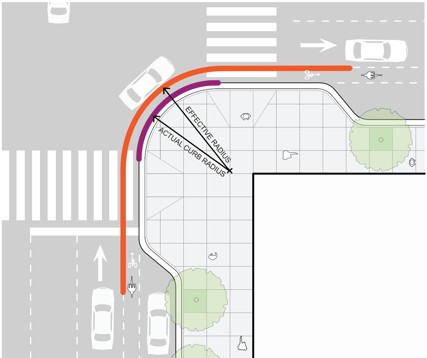
Figure 5-1 Actual vs Effective Radius
