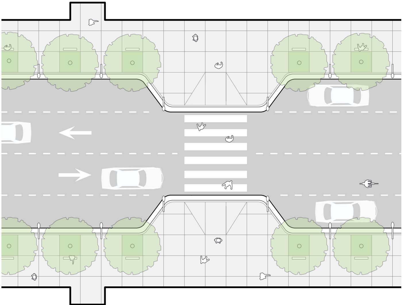
Figure 4-1 Neckdown with mid-block crossing
