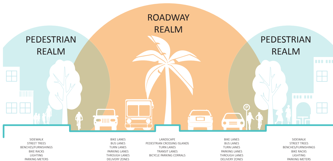
Figure 2-1 Cross-section elements
