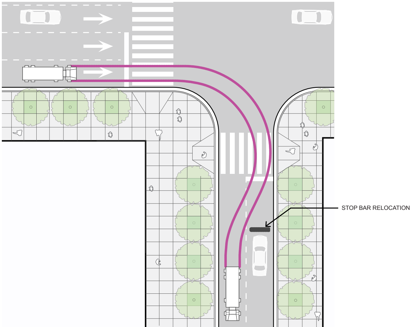
Figure 4-2 Stop Bar Relocation to Accommodate Large Vehicle Turns in a narrower Right-of-Way
