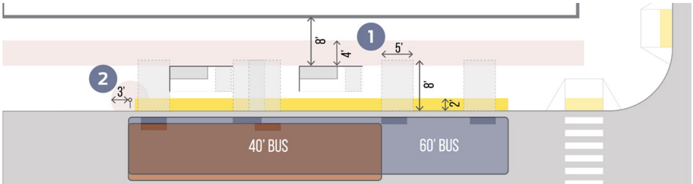
Figure 3-2 Recommended clear zones for bus stops - Source: NACTO
