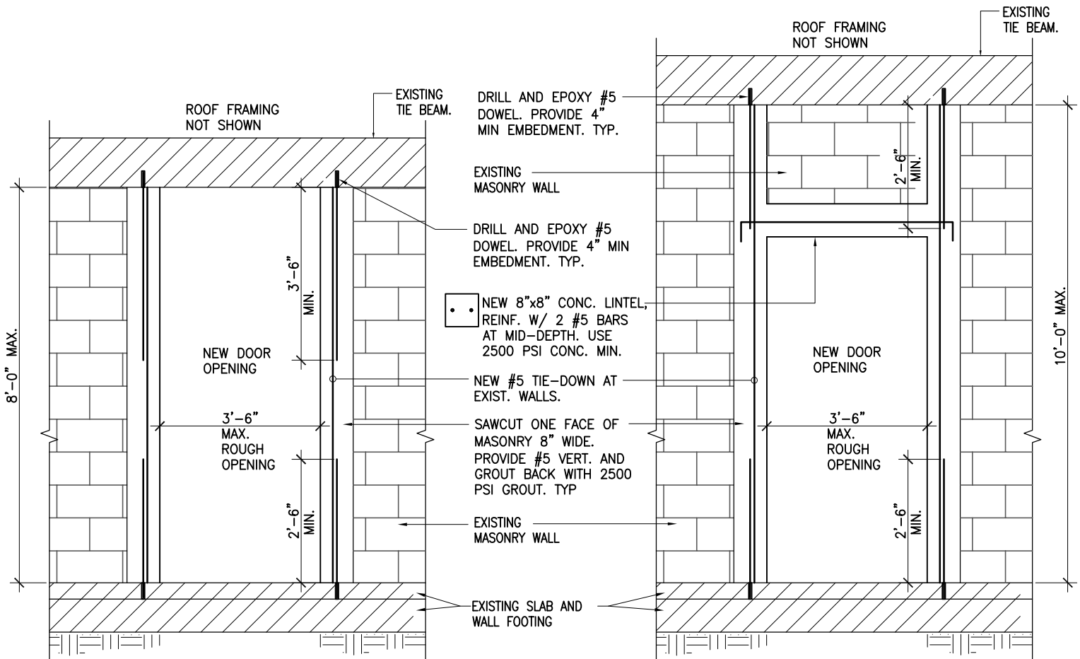
NEW DOOR OPENING DETAIL 1 ELEVATION
