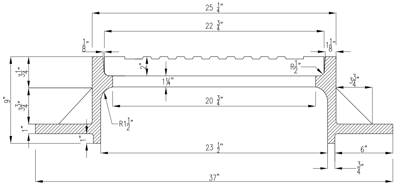
FRAME SECTION
