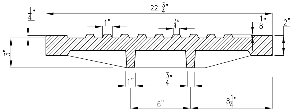
COVER SECTION
