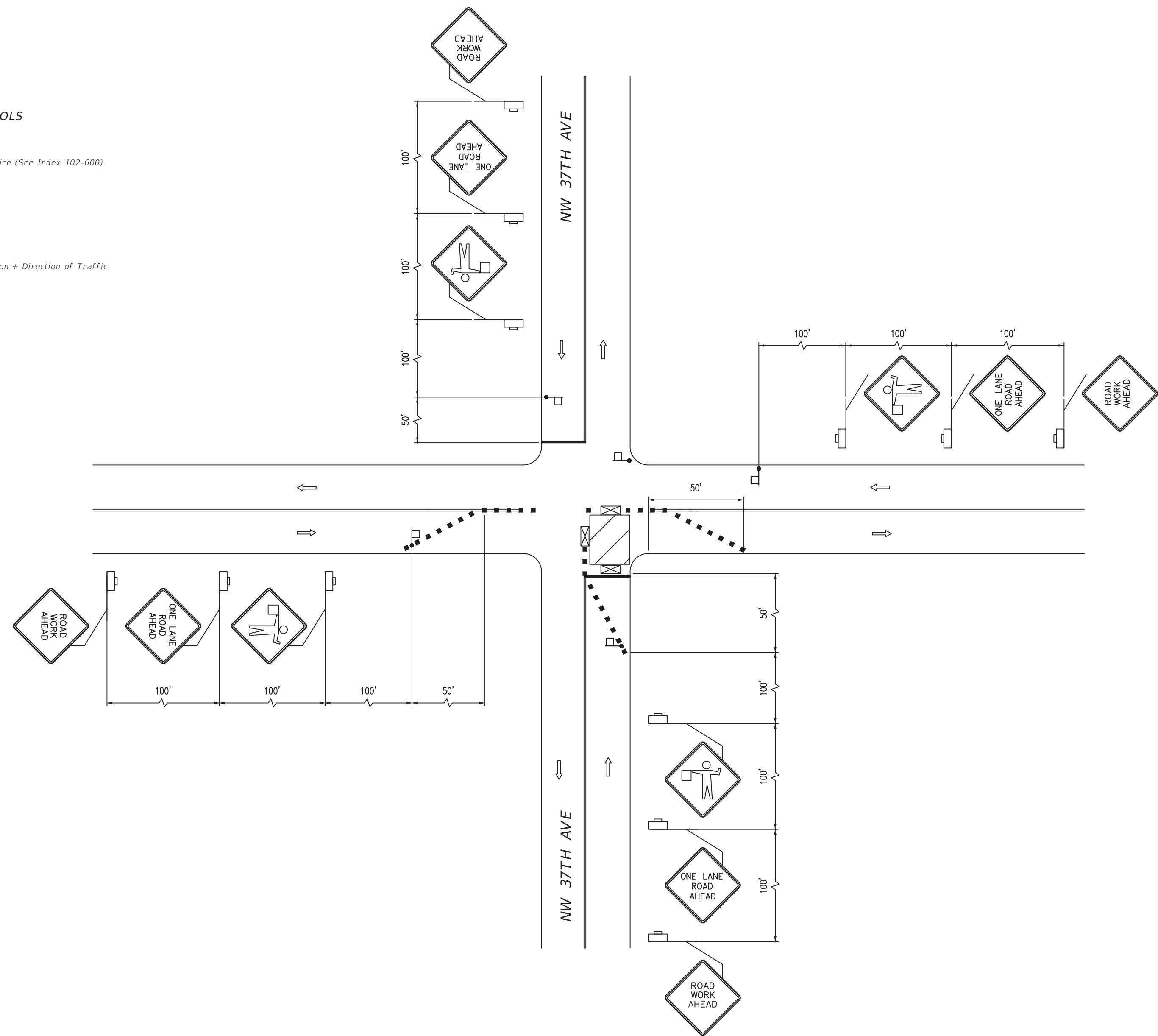
CLOSURE AT SIDE OF INTERSECTION - STANDARD DETAIL 1
