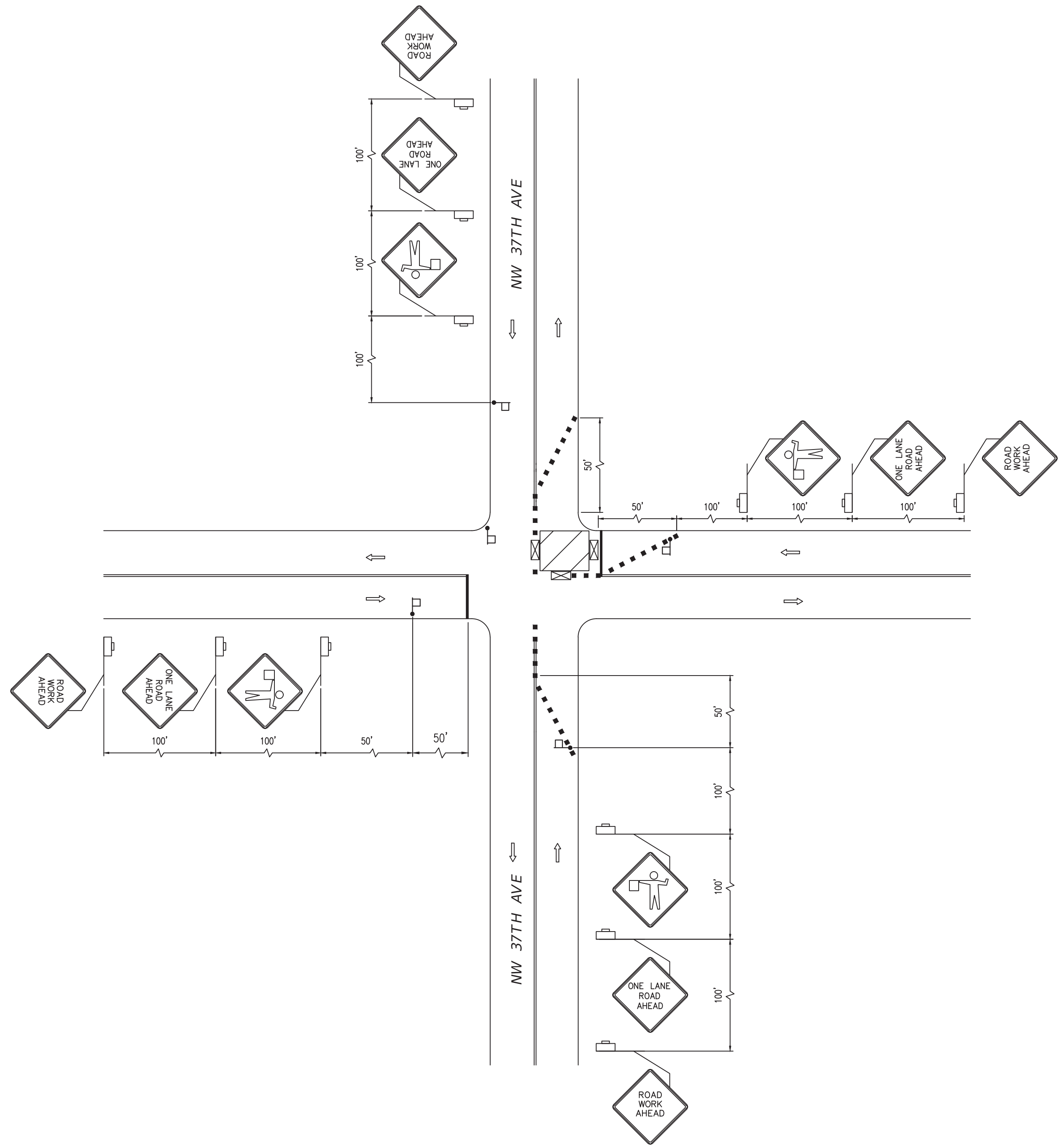
CLOSURE AT SIDE OF INTERSECTION - STANDARD DETAIL 2
