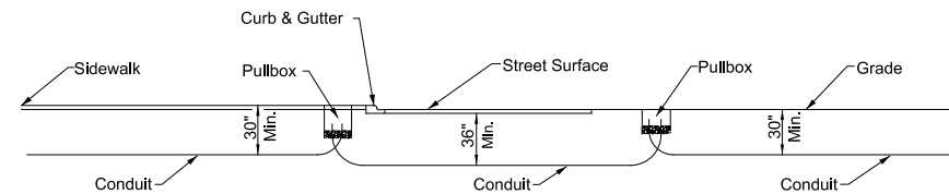
UNDER ROADWAY SECTION
