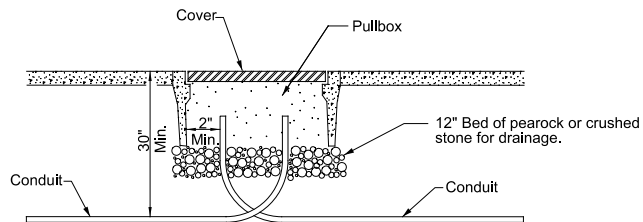
PULLBOX ENTRY OF CONDUIT UNDER SIDEWALKS
