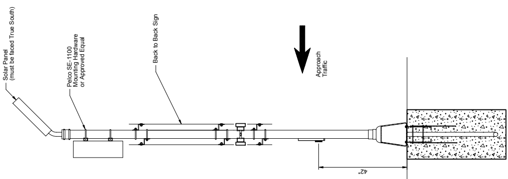
SOLAR POWERED RRFB SIDE VIEW
