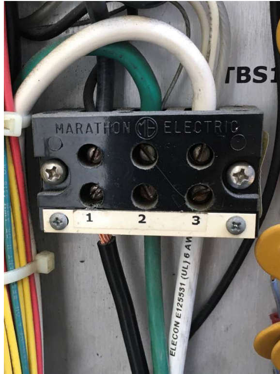
Figure 5 TBS1 Terminal Inside the Traffic Signal Cabinet
