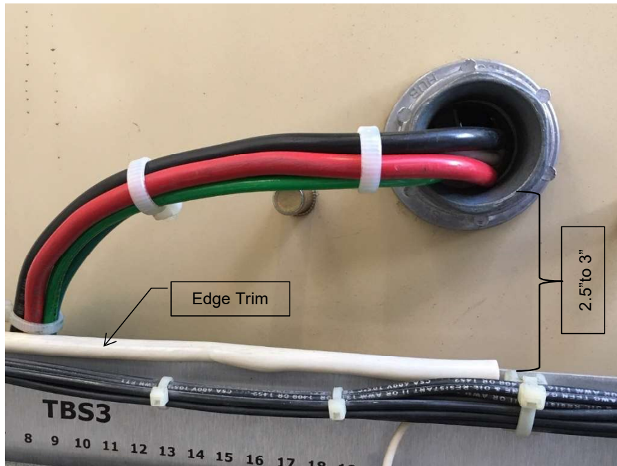
Figure 1 Ground hub Inside Traffic Signal Cabinet
