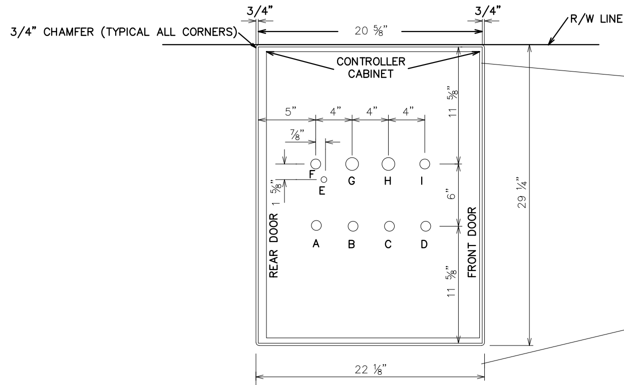
CONTROLLER CABINET AND CONDUIT ARRANGEMENT DETAIL
