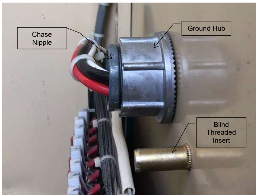
Figure 3 Ground Hub and Chase Nipple Inside Traffic Signal Cabinet
