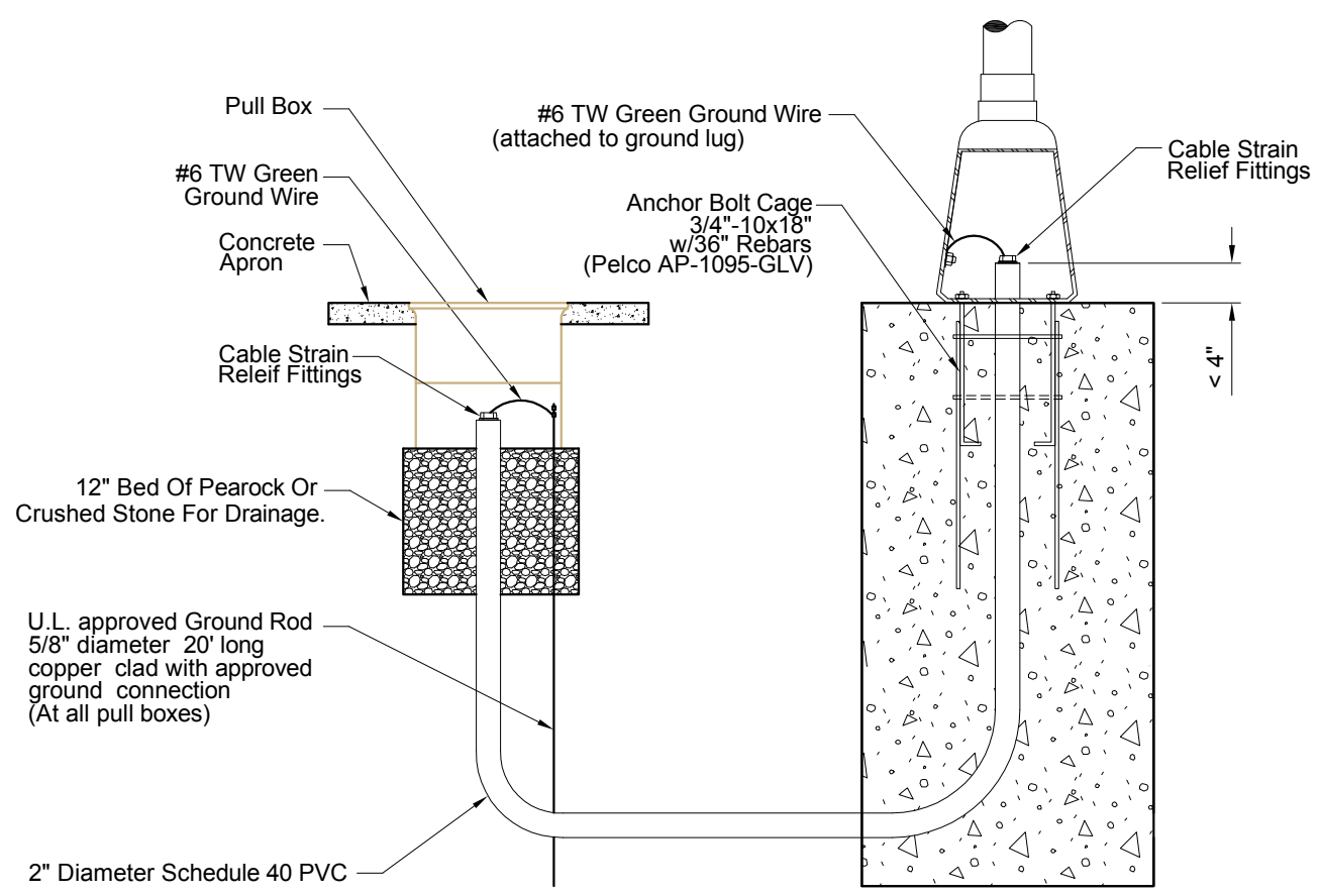
POLE GROUND DETAIL SOLAR POWERED BEACON
