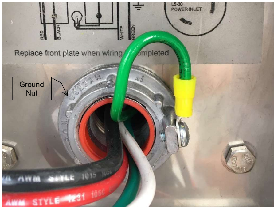
Figure 2 Ground Nut inside Transfer Switch Enclosure
