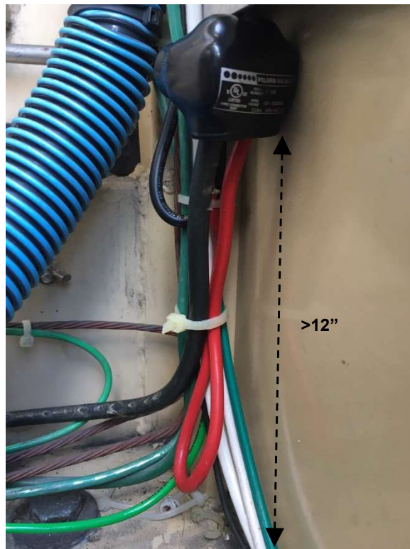
Figure 4 Splice Connector Inside Traffic Signal Cabinet
