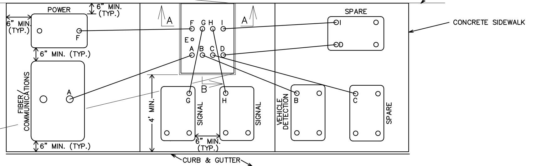
CONTROLLER CABINET AND PULL BOX DETAIL
