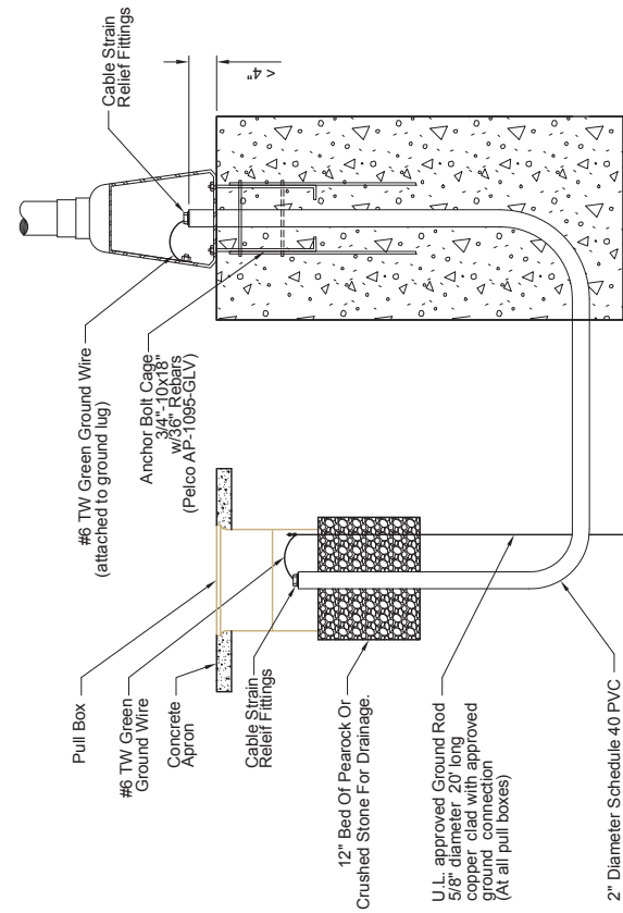
POLE GROUND DETAIL SOLAR POWERED BEACON
