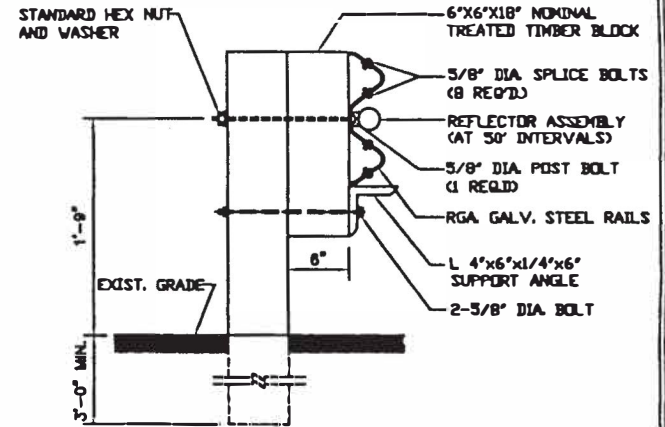
SUPPORT POST DETAIL N.T.S.
