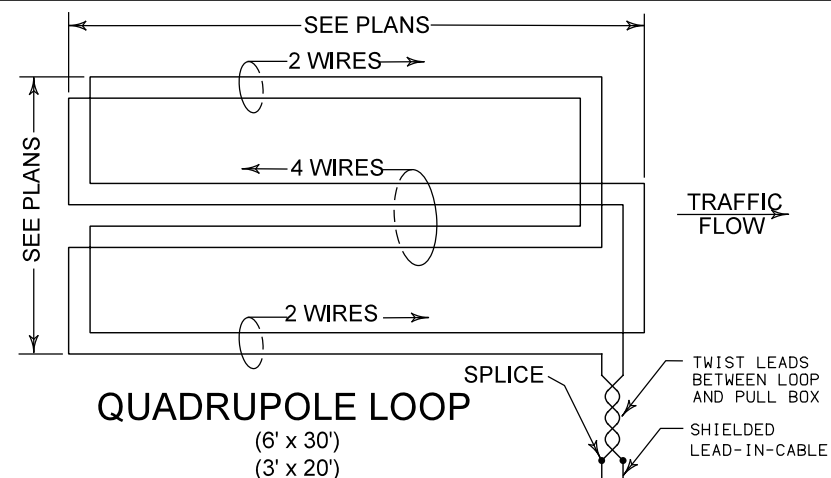
TYPICAL DETECTOR LOOP WIRE CONFIGURATION
