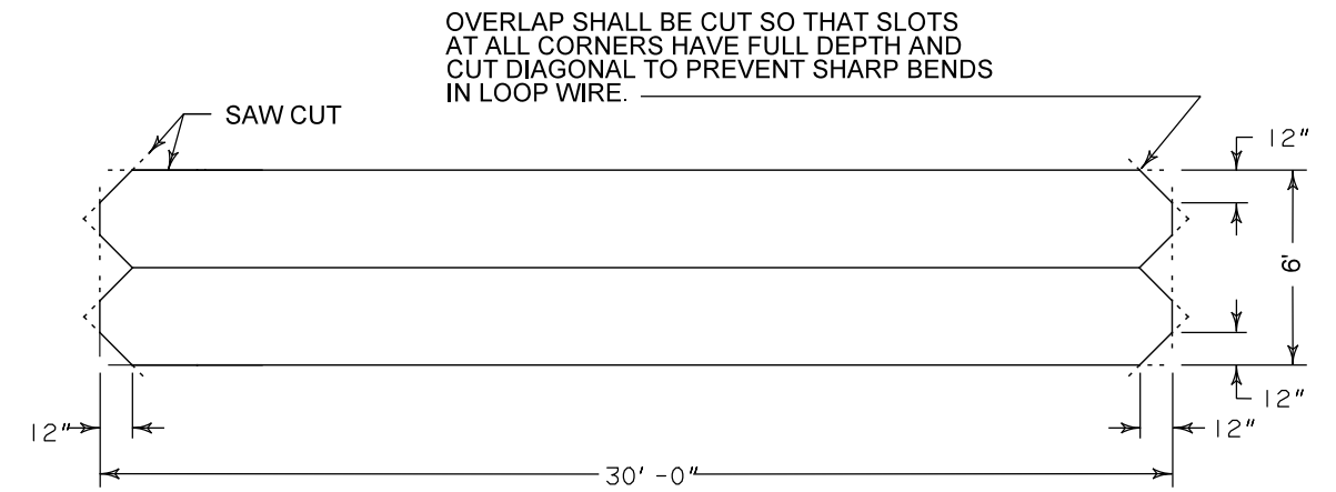
TYPICAL "TYPE F" VEHICLE INDUCTIVE LOOP
