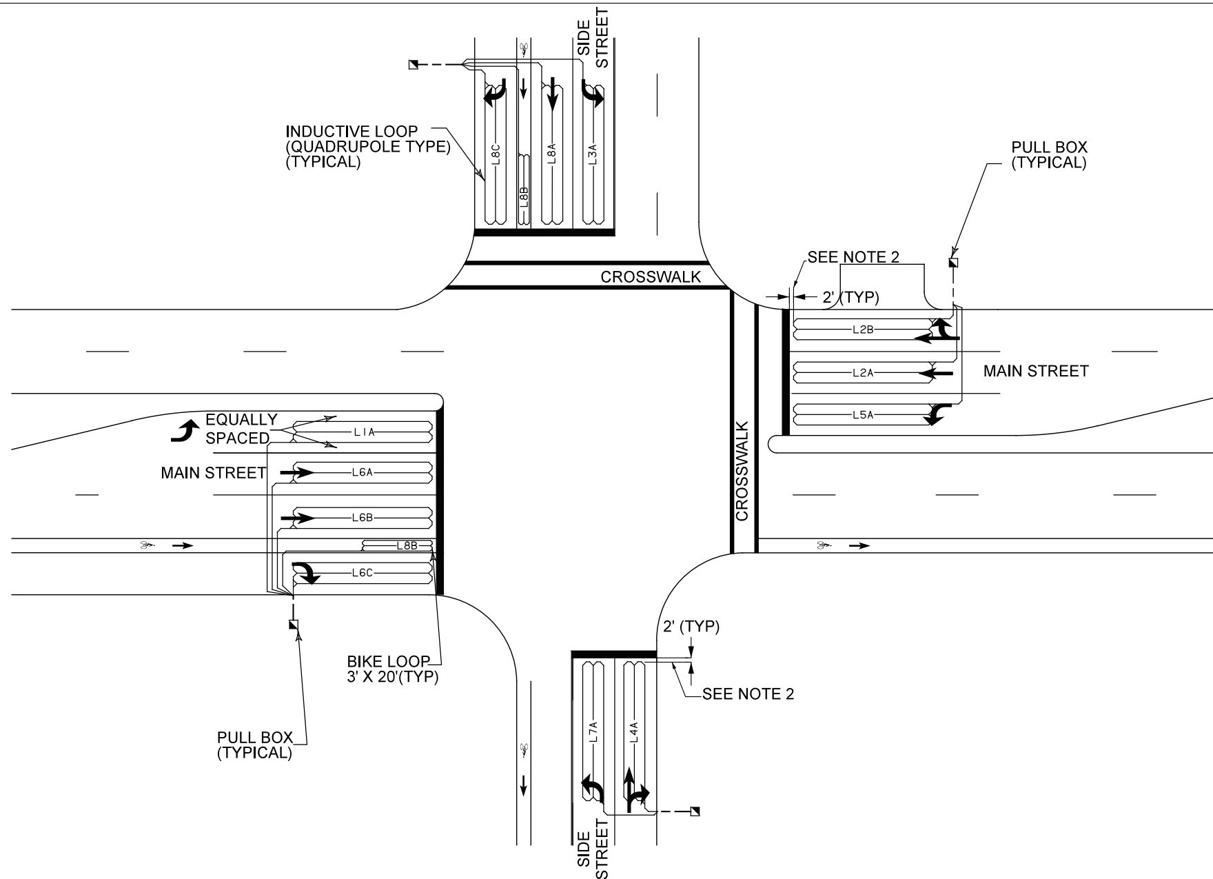
TYPICAL INDUCTIVE LOOP PLACEMENT
