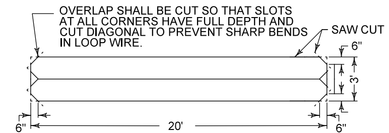
TYPICAL "TYPE F" MODIFIED BICYCLE INDUCTIVE LOOP
